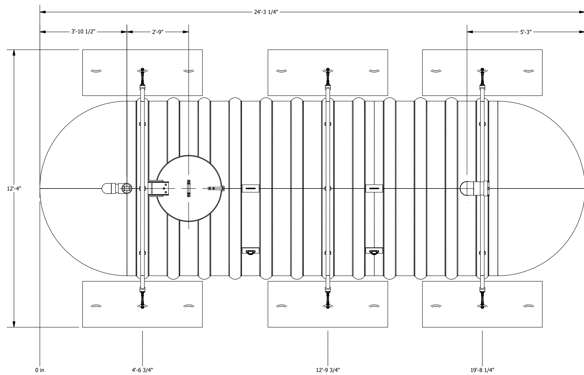
PLAN VIEW
