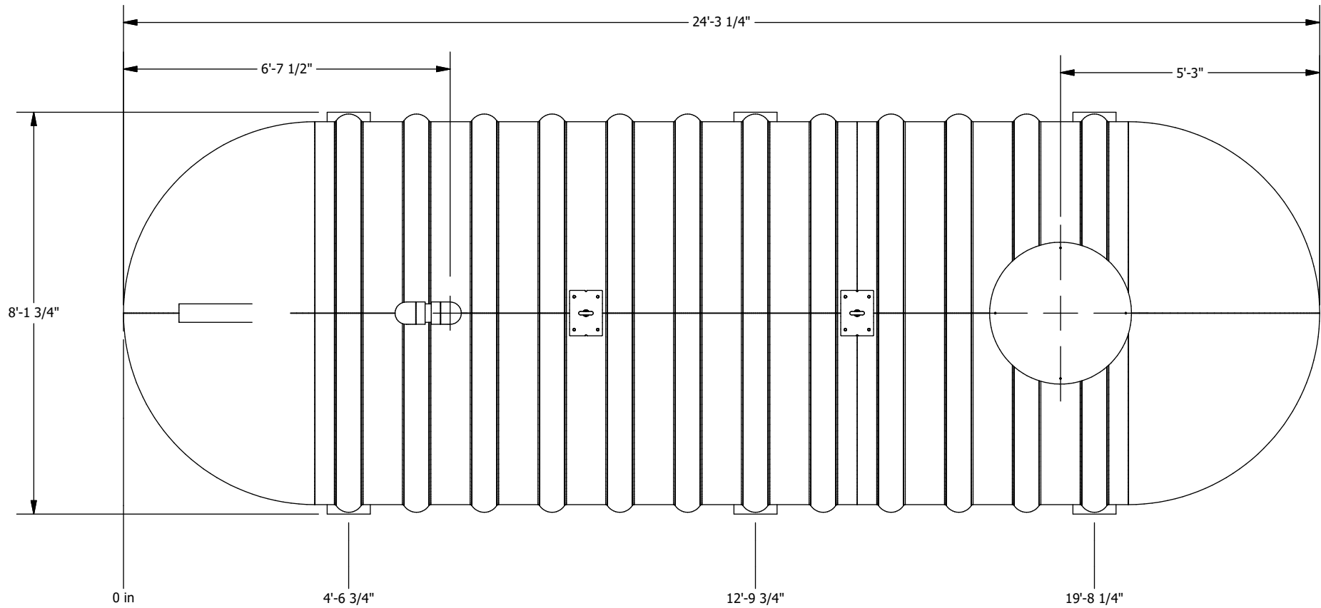
PLAN VIEW
