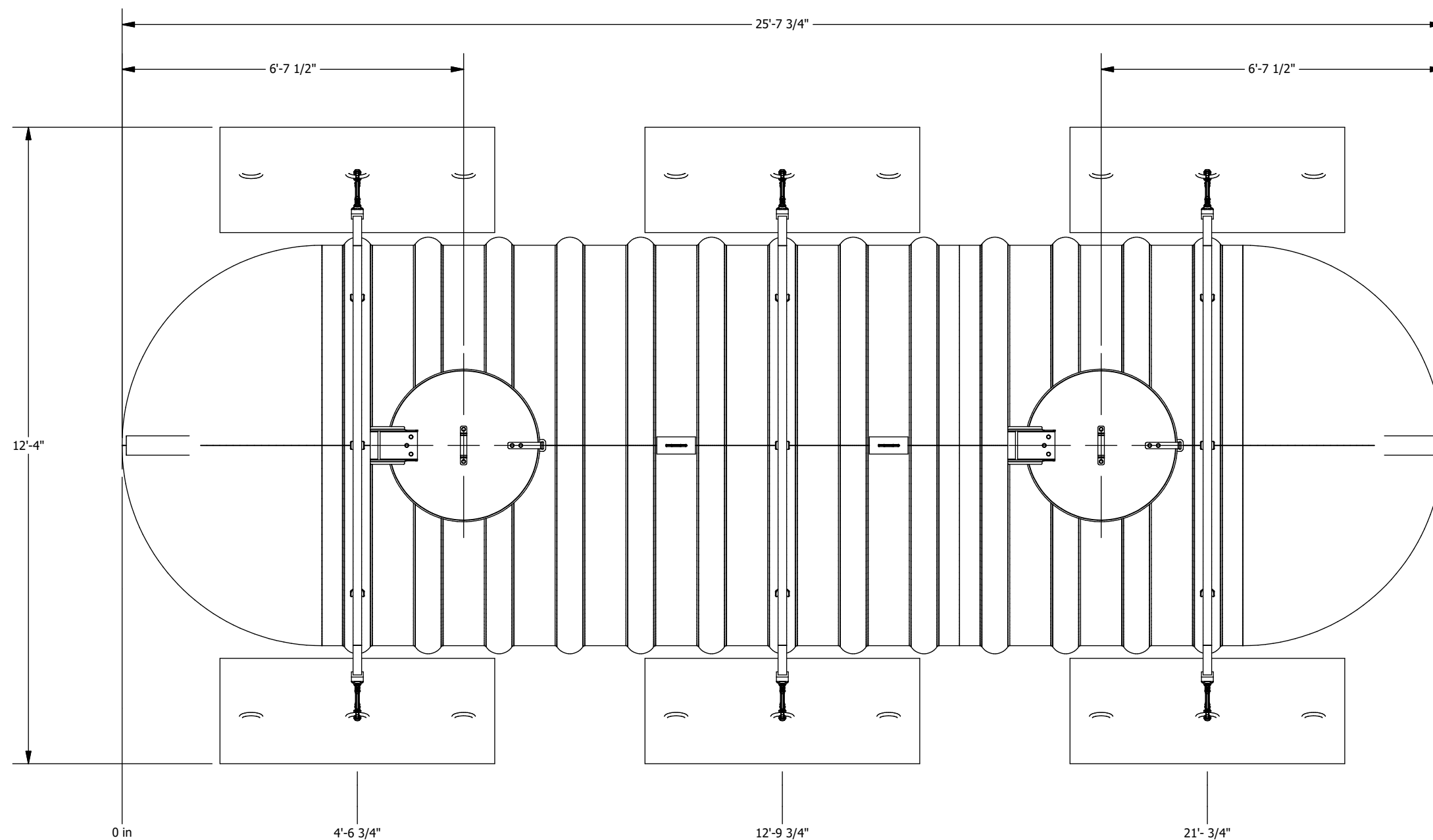
PLAN VIEW
