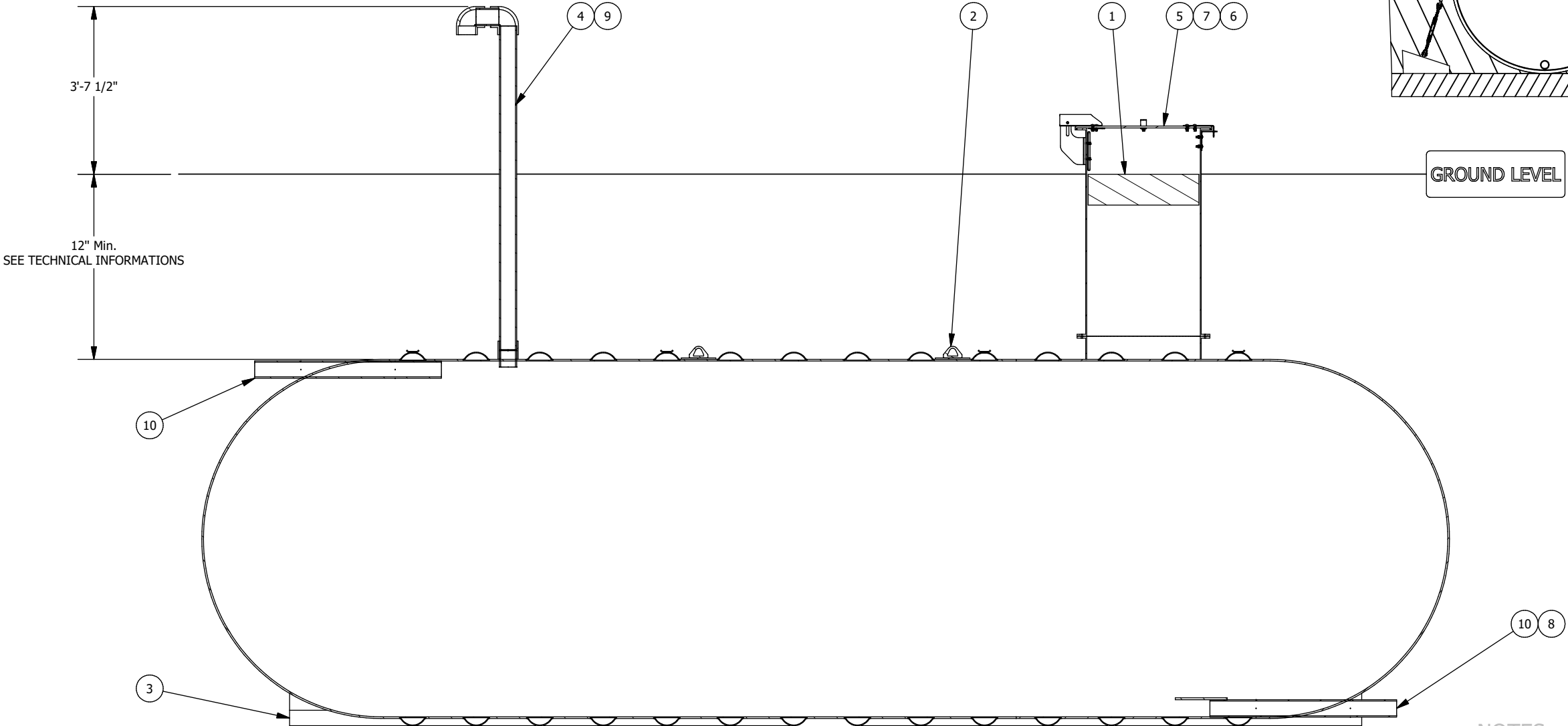
SECTION ELEVATION VIEW
