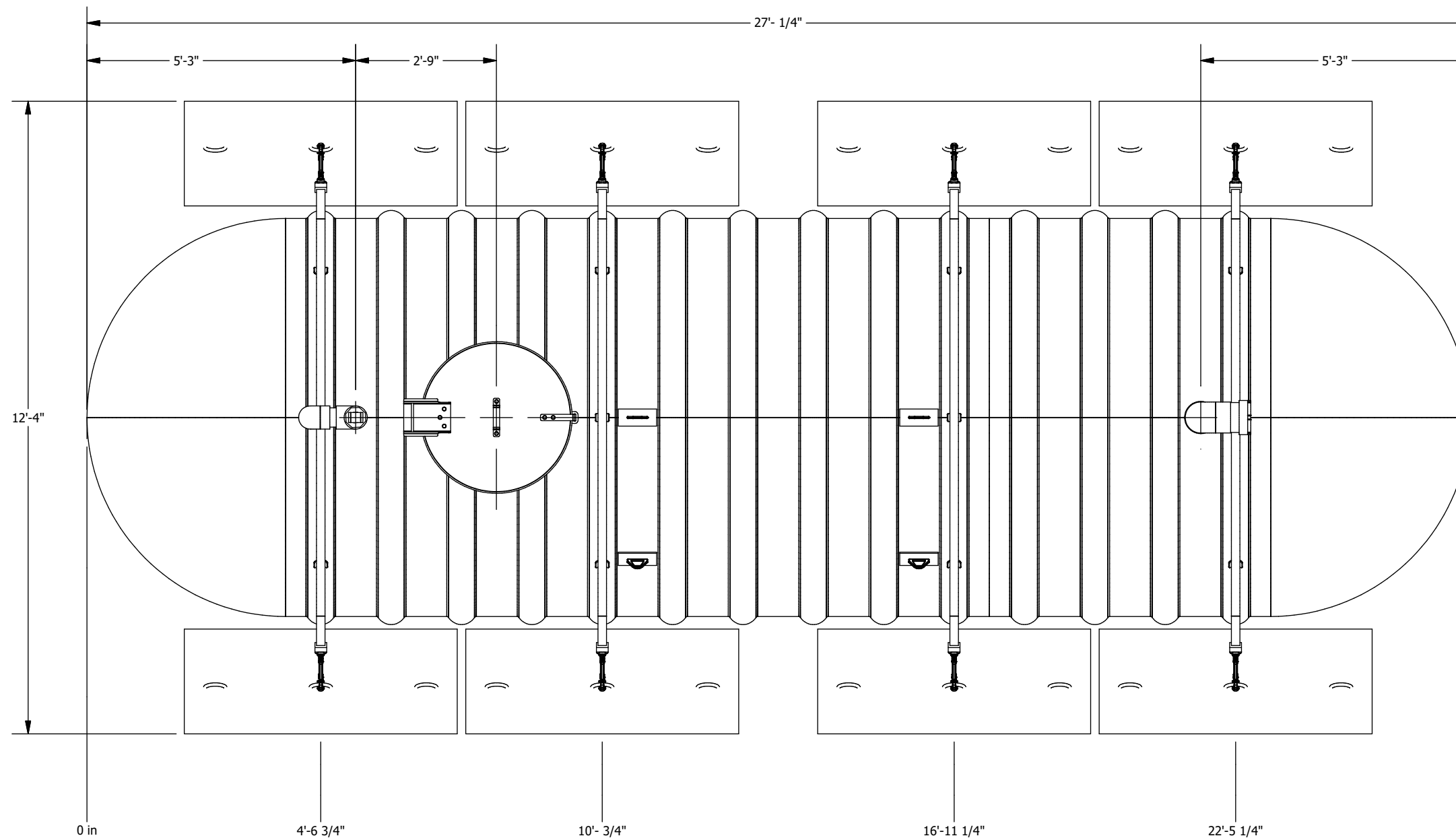
PLAN VIEW
