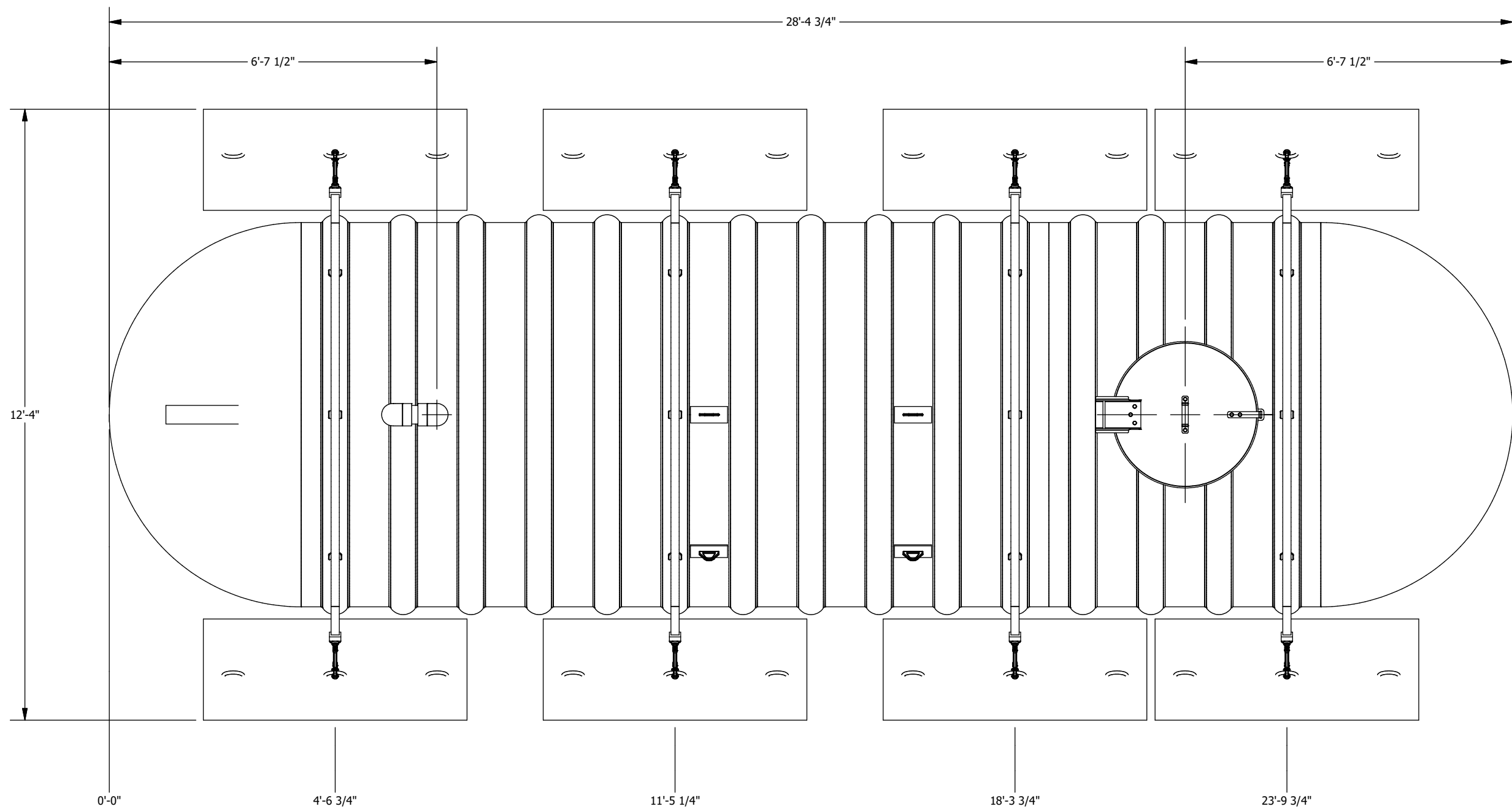
PLAN VIEW
