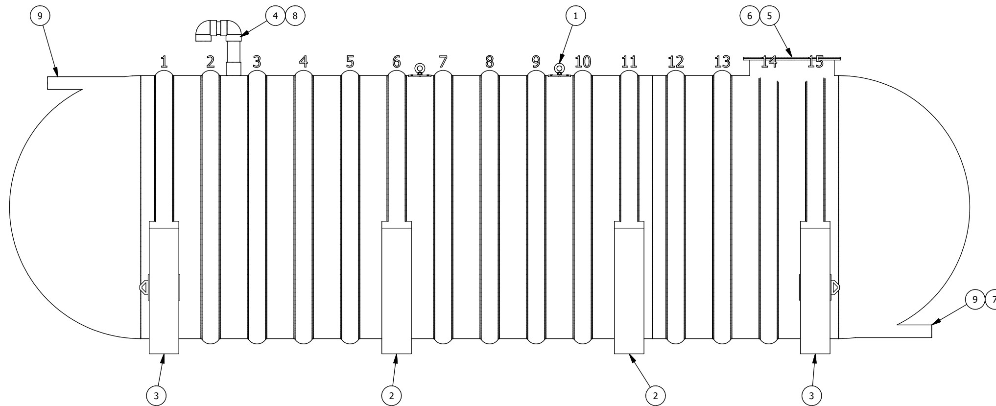
ELEVATION VIEW
