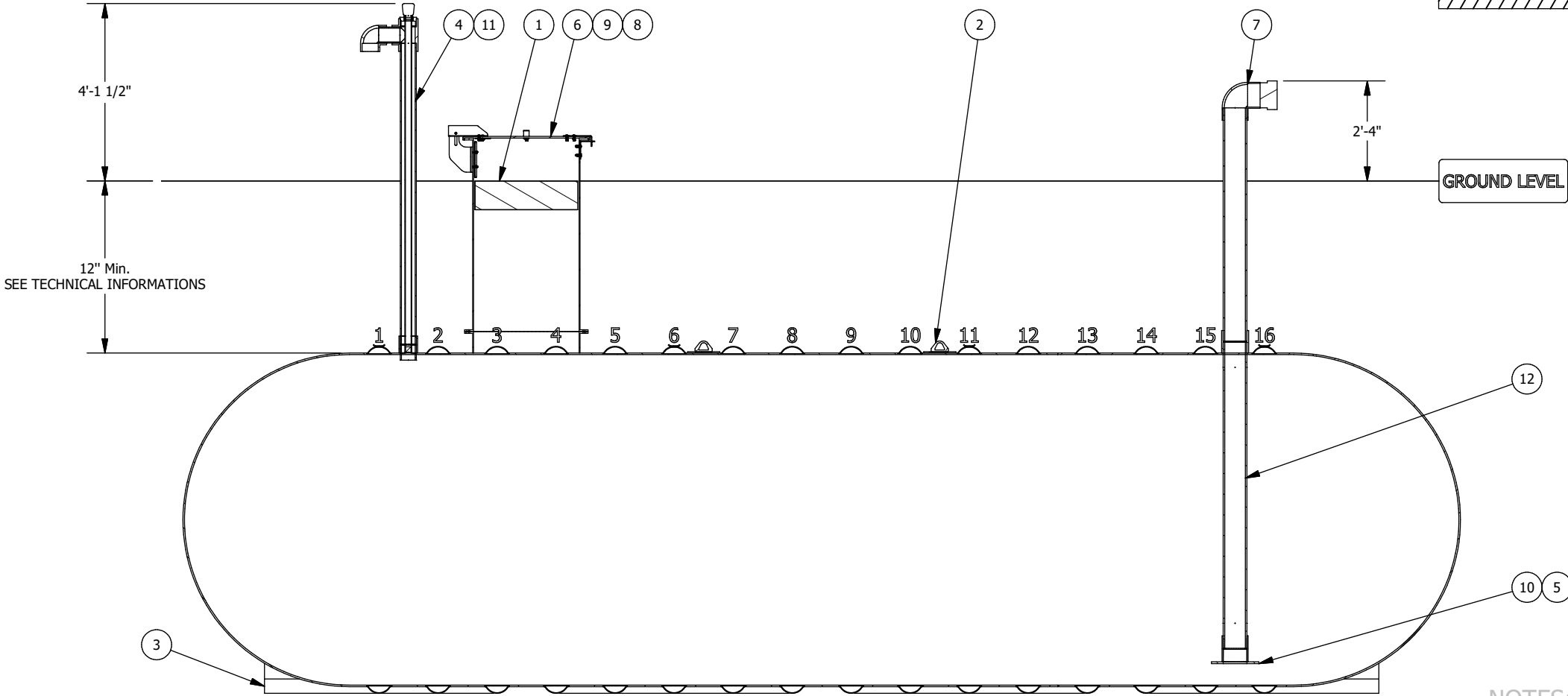
SECTION ELEVATION VIEW
