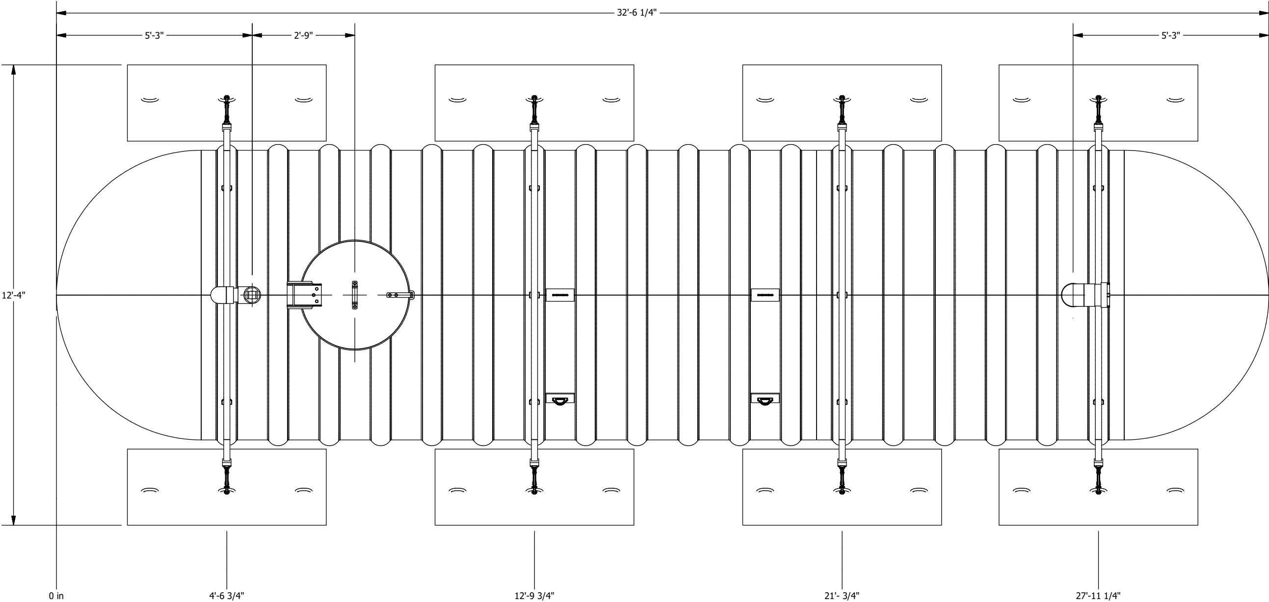
PLAN VIEW
