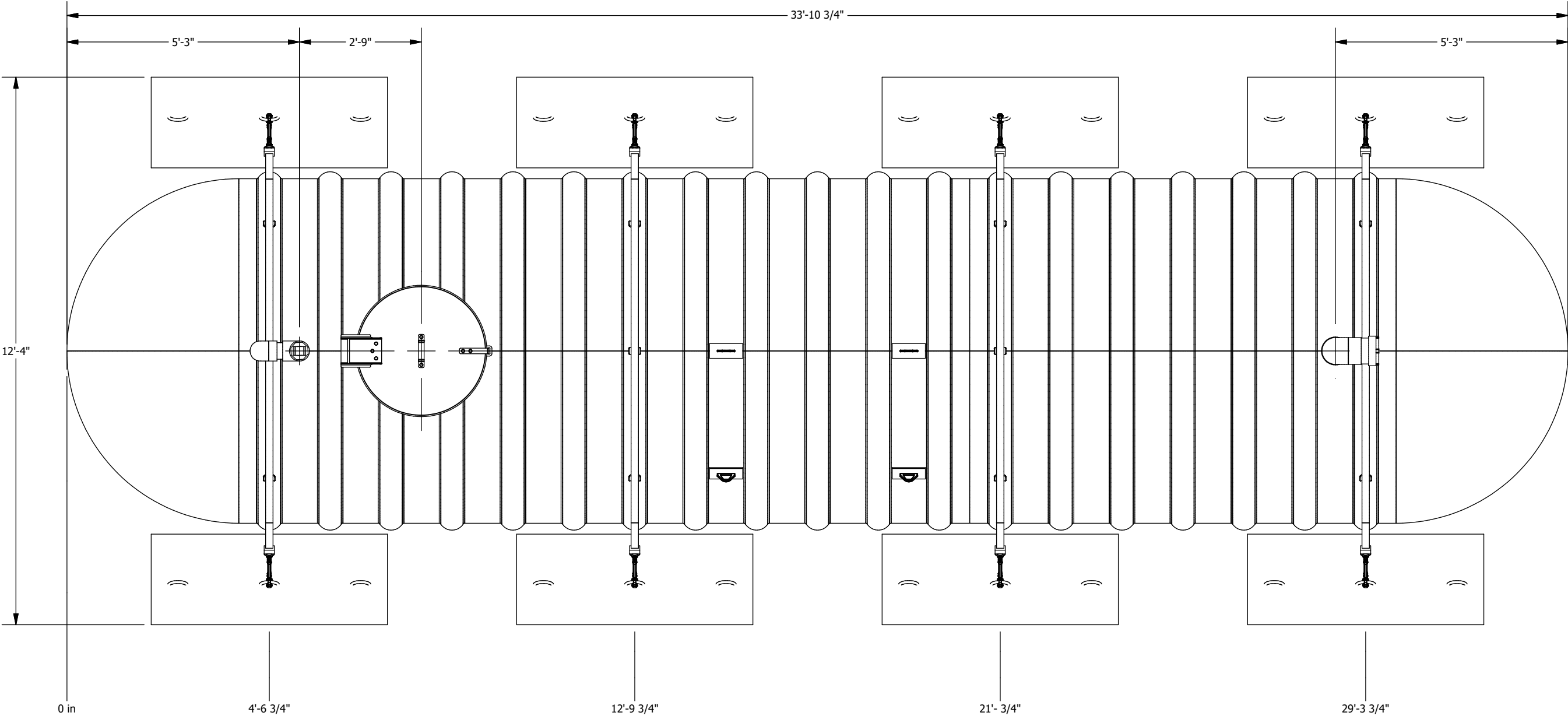
PLAN VIEW
