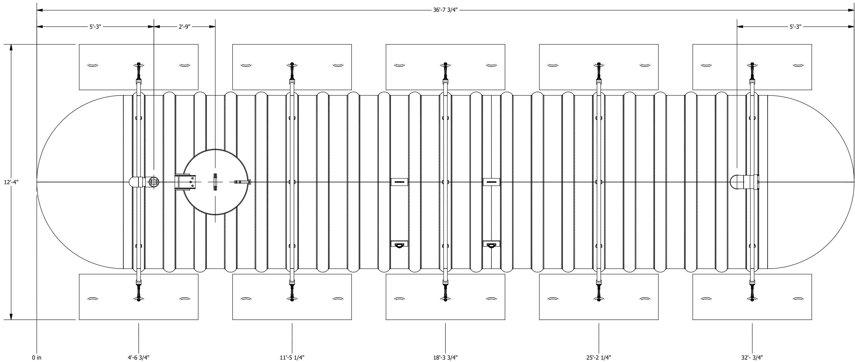
PLAN VIEW
