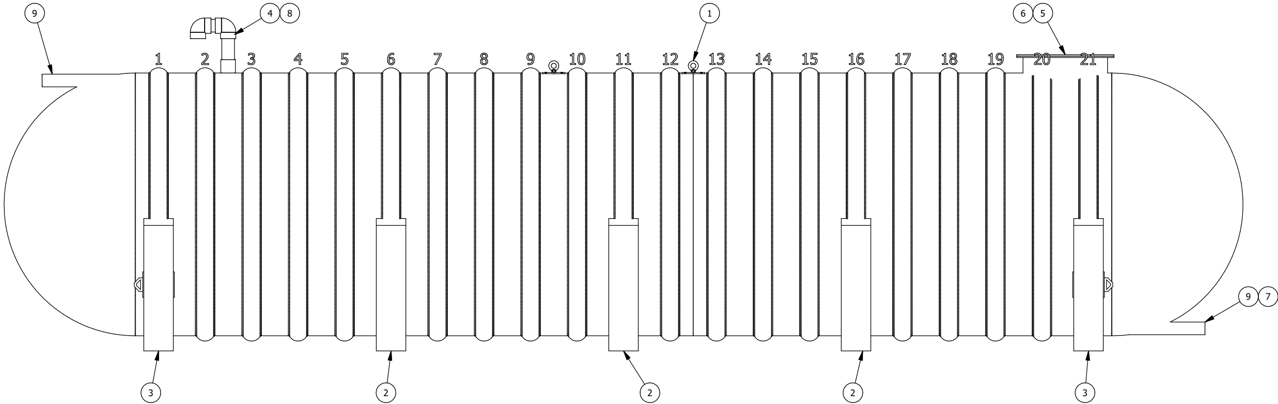
ELEVATION VIEW
