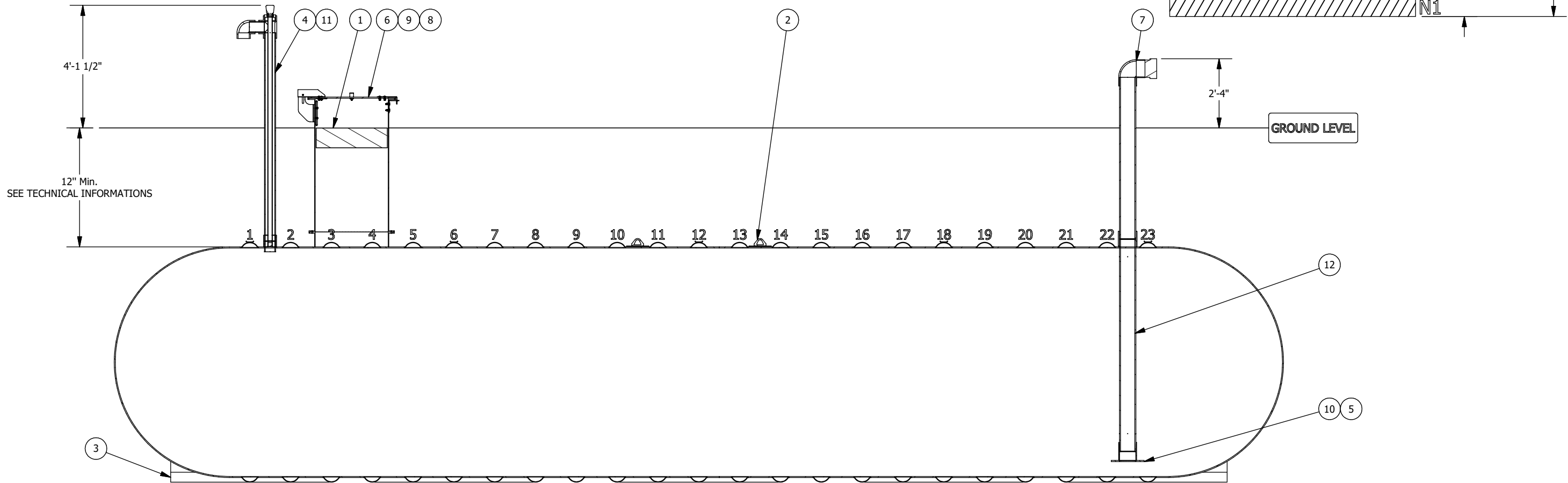
SECTION ELEVATION VIEW
