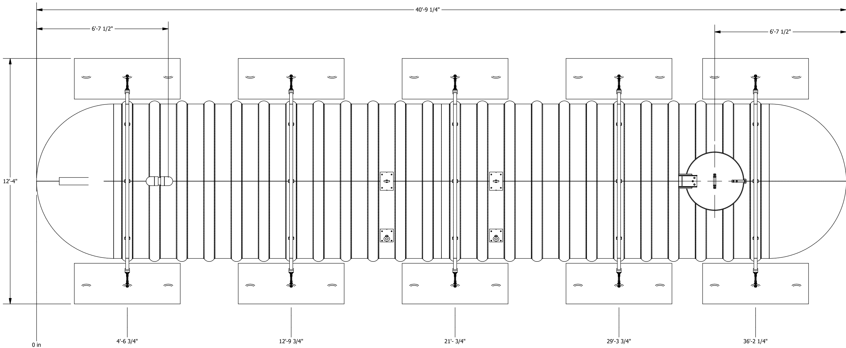
PLAN VIEW
