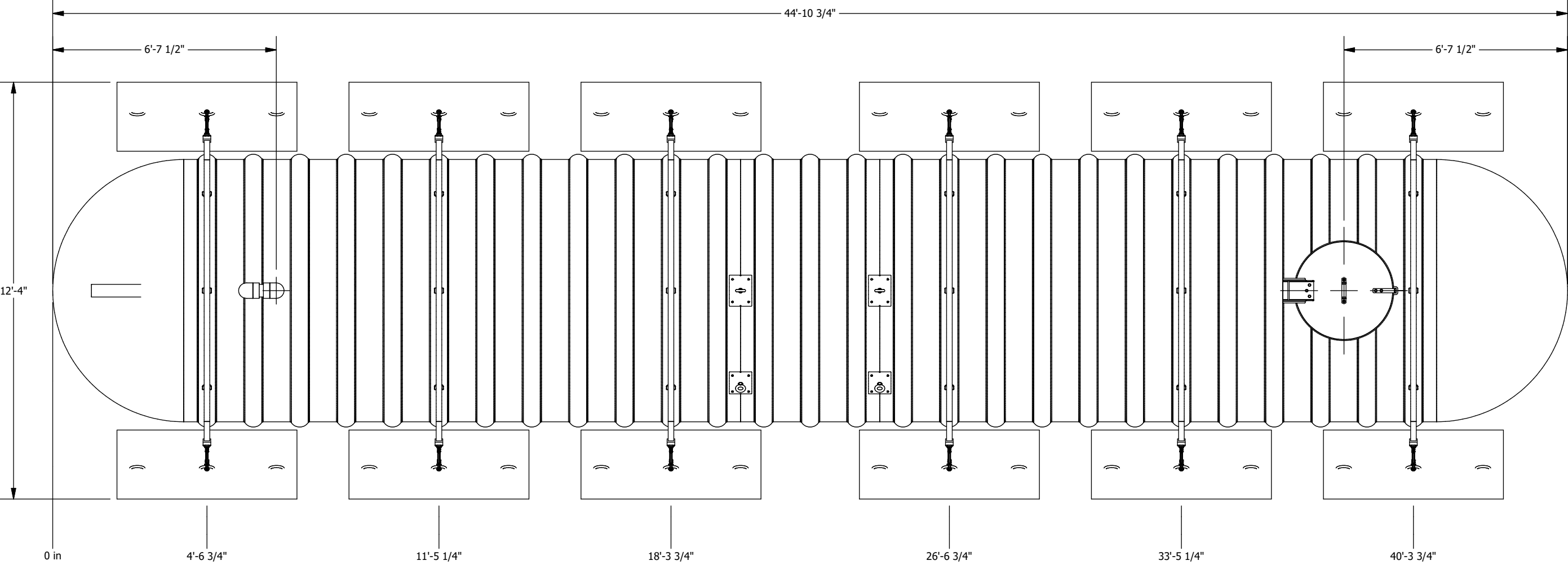
PLAN VIEW
