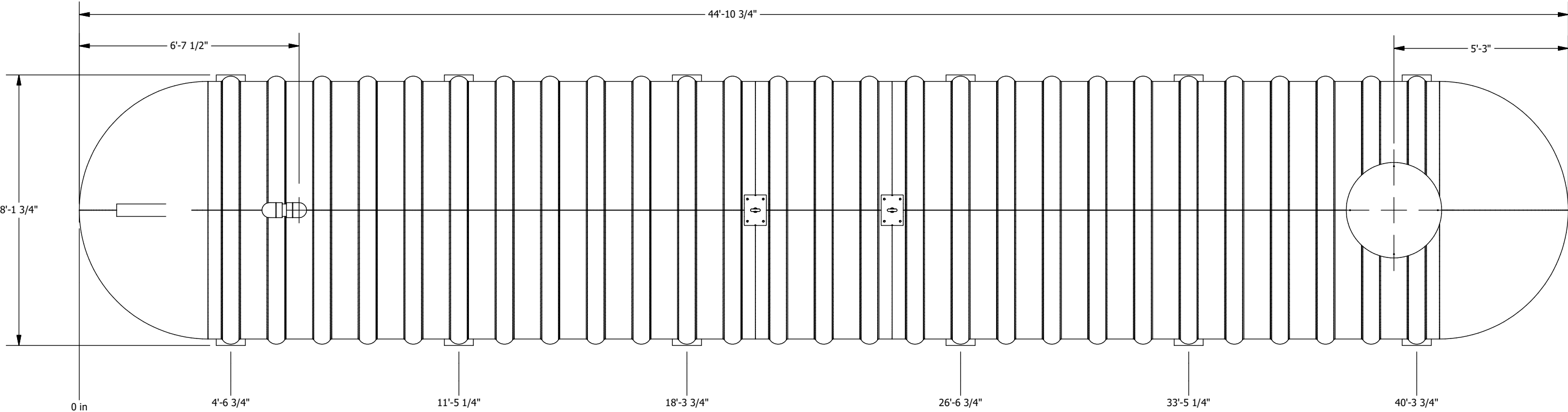
PLAN VIEW
