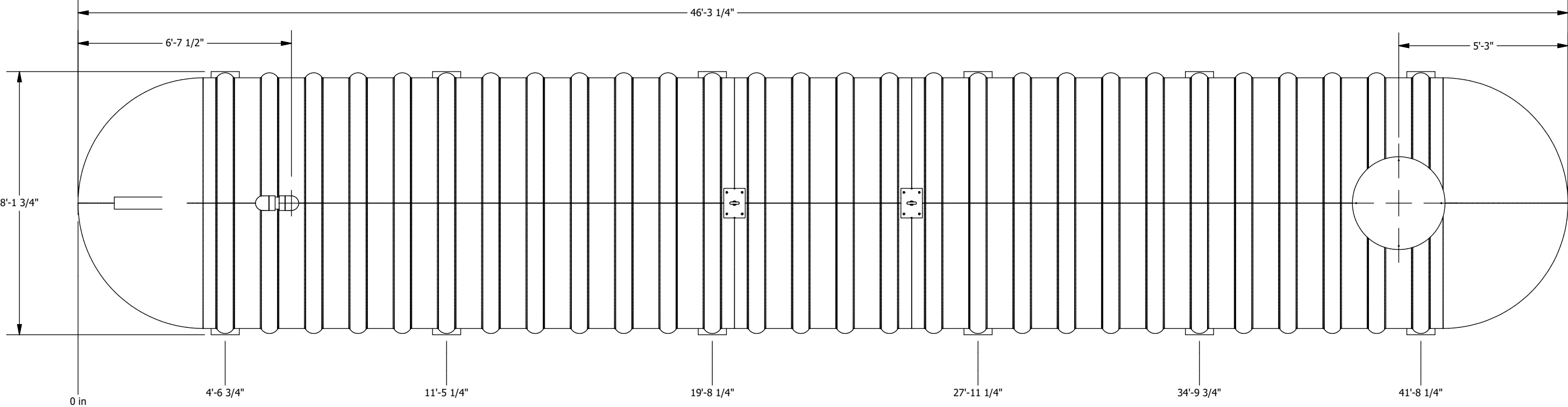
PLAN VIEW
