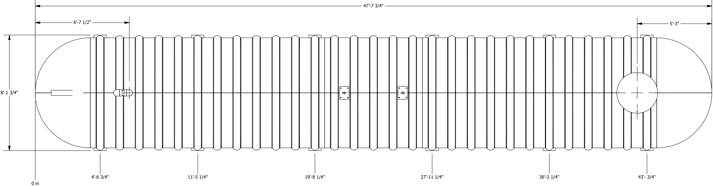
PLAN VIEW
