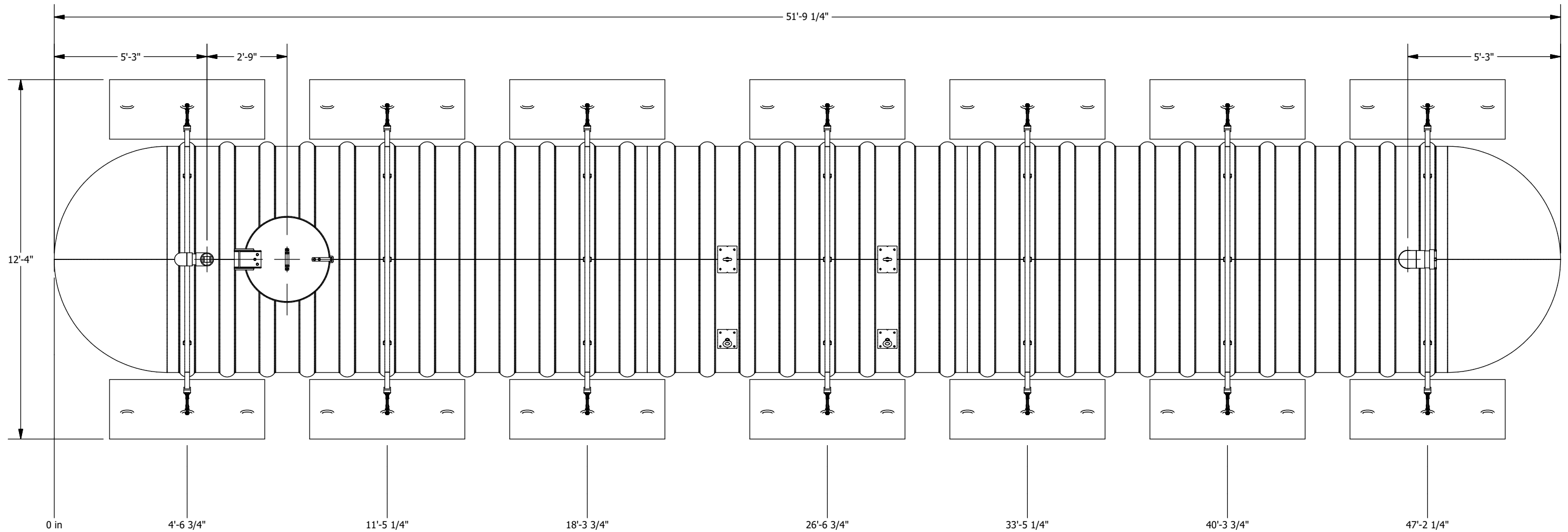
PLAN VIEW
