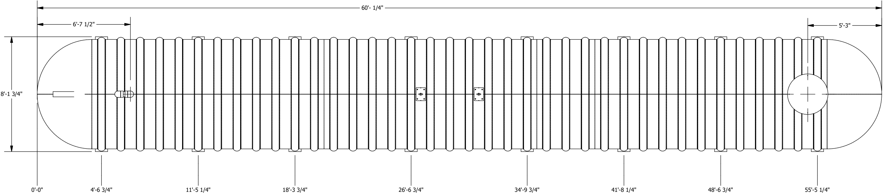
PLAN VIEW
