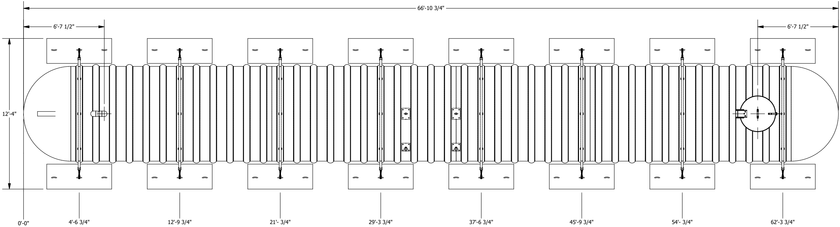
PLAN VIEW
