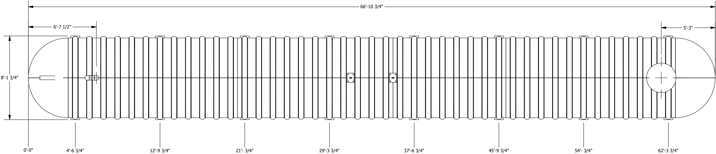
PLAN VIEW
