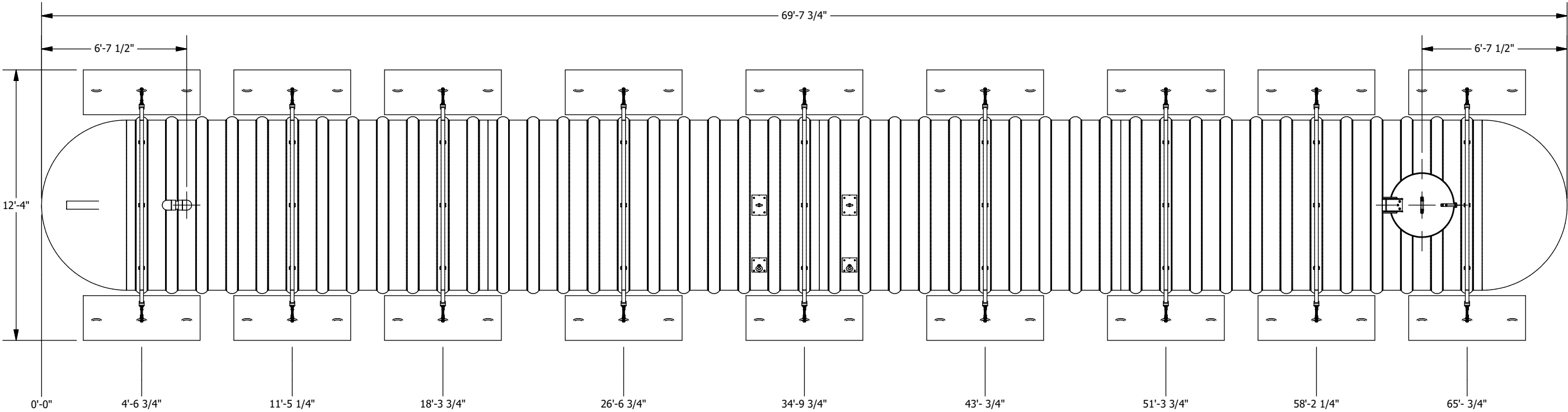
PLAN VIEW
