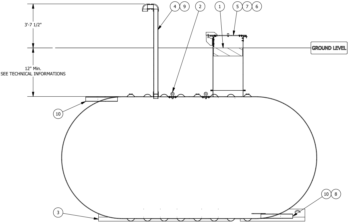
SECTION ELEVATION VIEW
