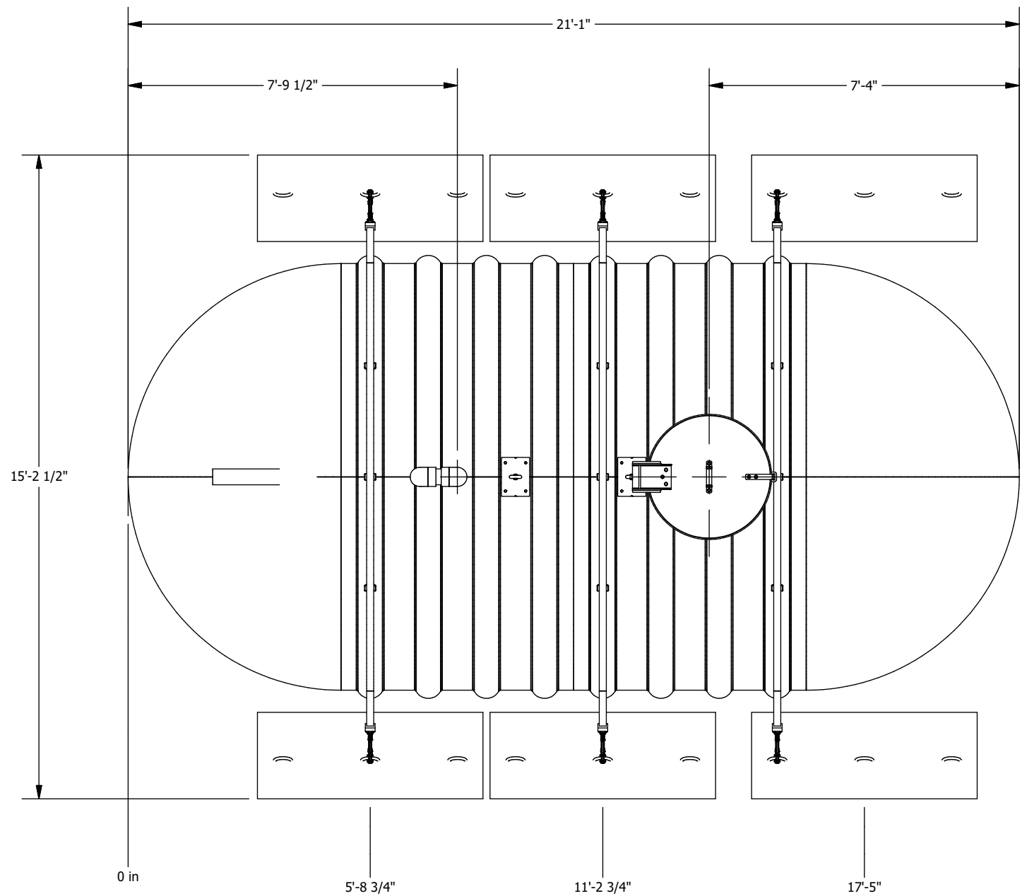
PLAN VIEW
