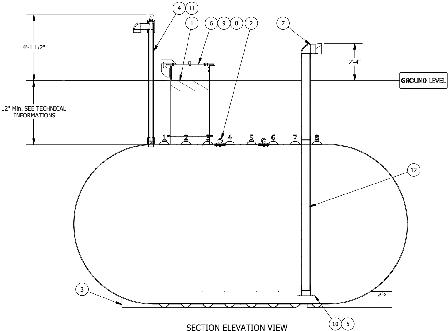
SECTION ELEVATION VIEW
