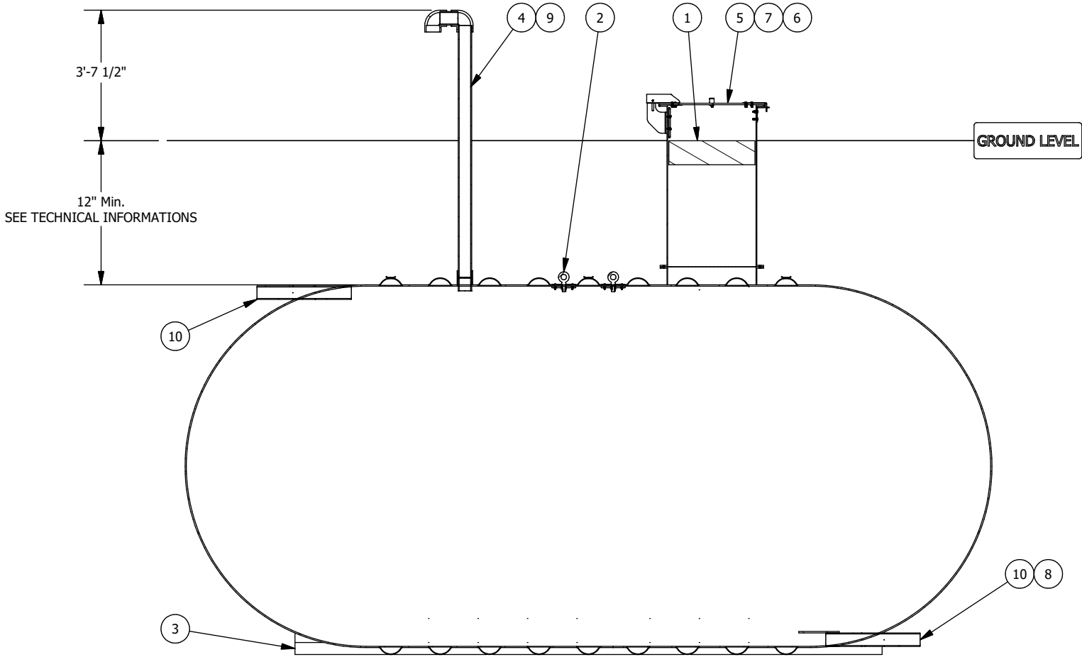
SECTION ELEVATION VIEW
