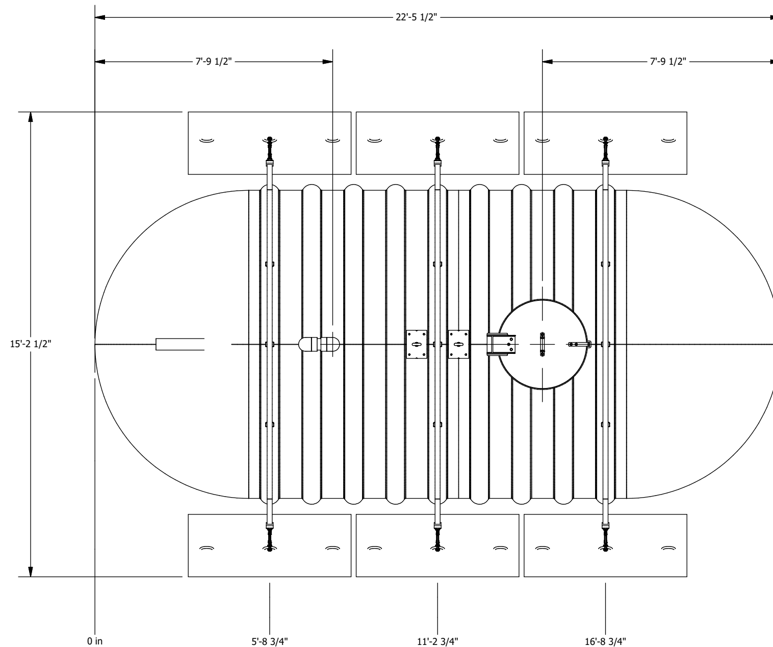
PLAN VIEW
