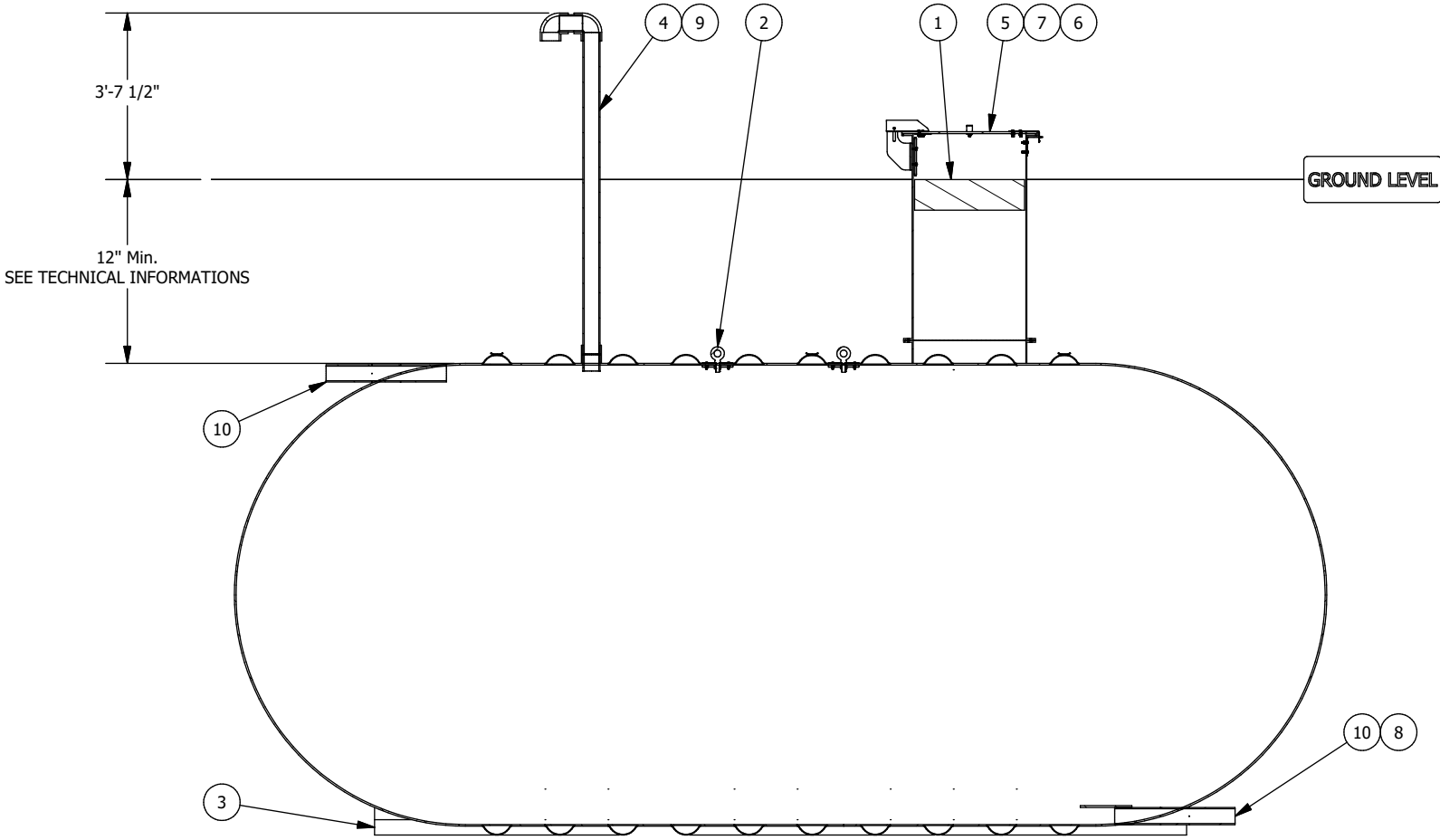
SECTION ELEVATION VIEW
