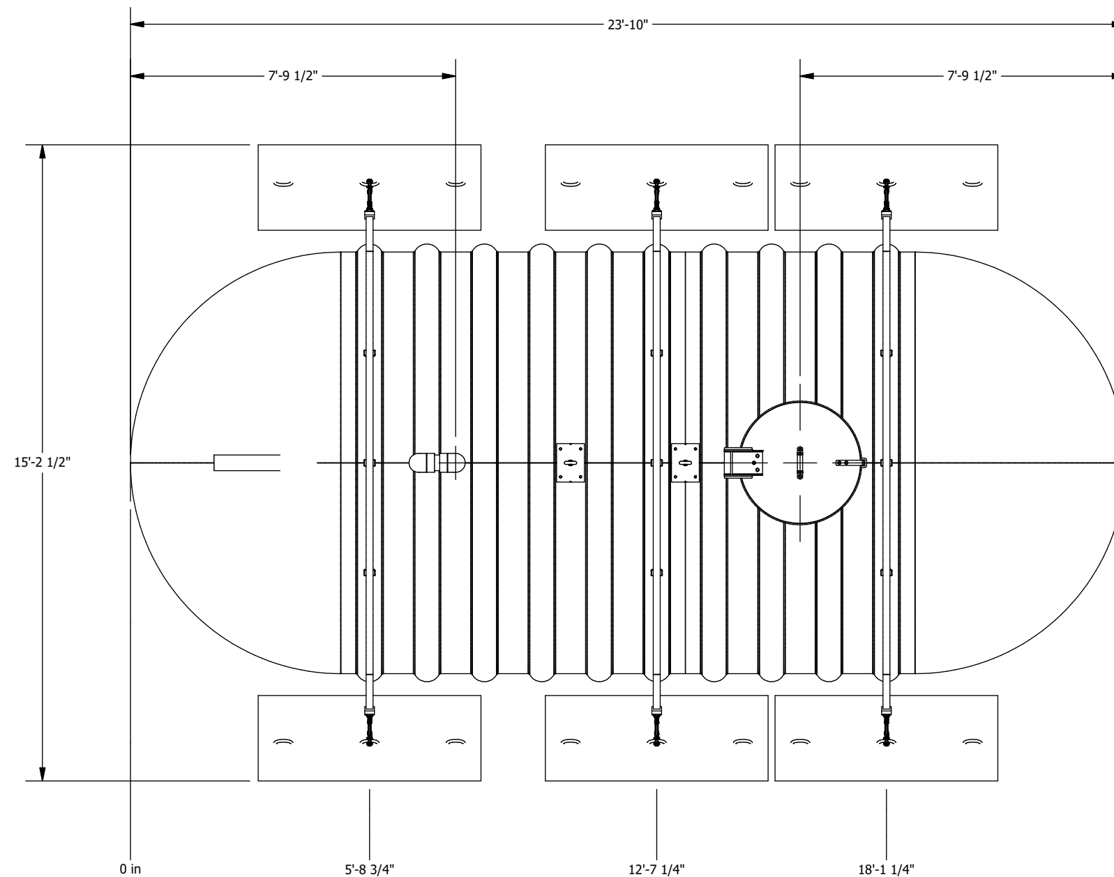
PLAN VIEW
