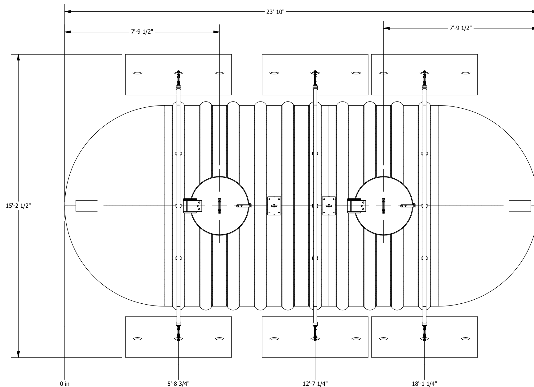
PLAN VIEW
