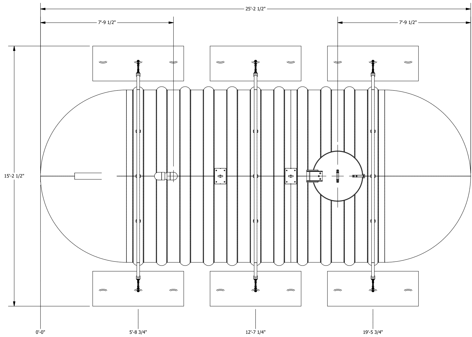
PLAN VIEW
