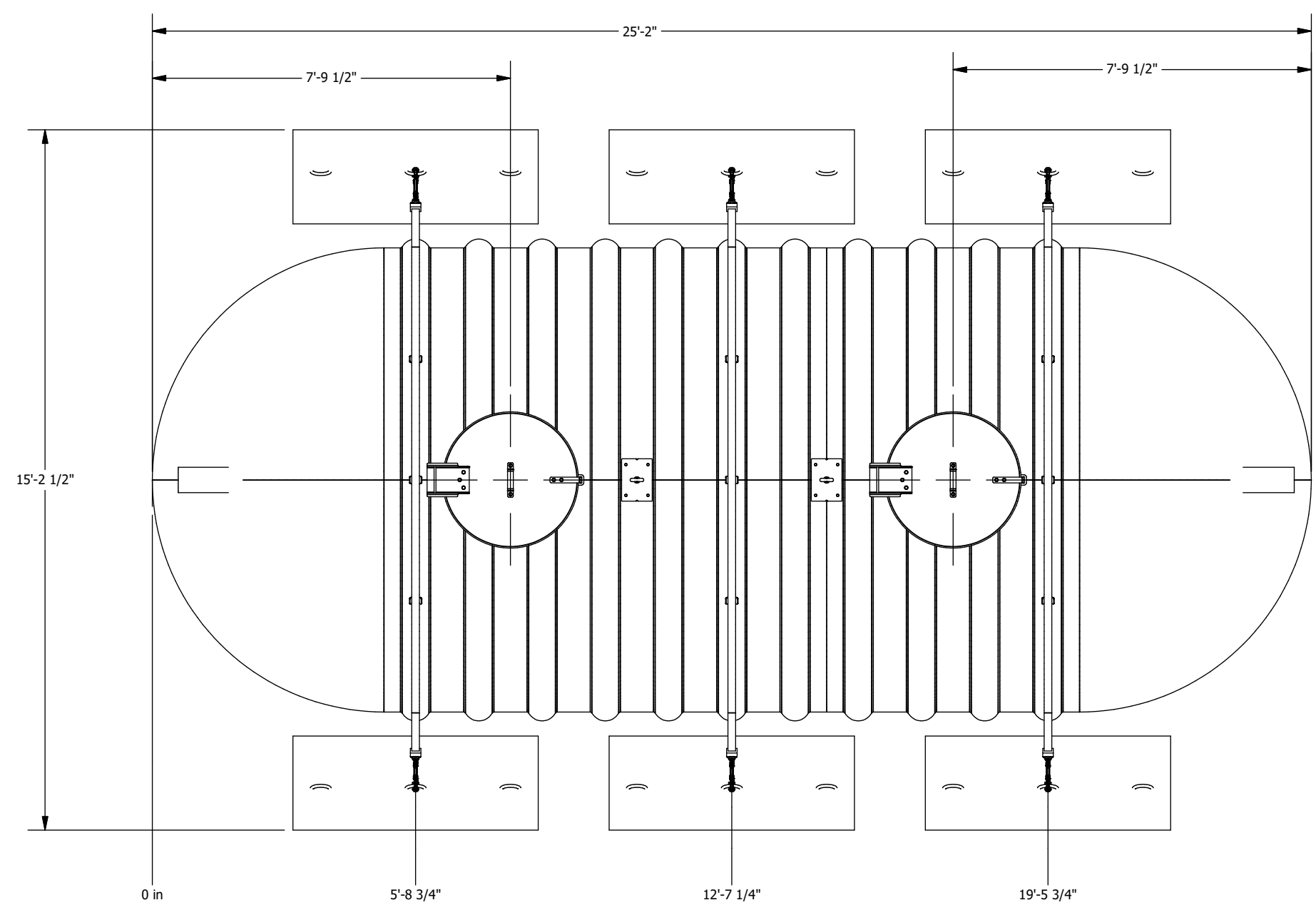
PLAN VIEW
