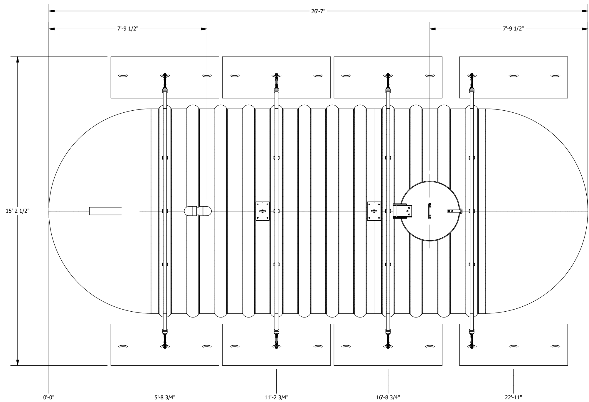
PLAN VIEW
