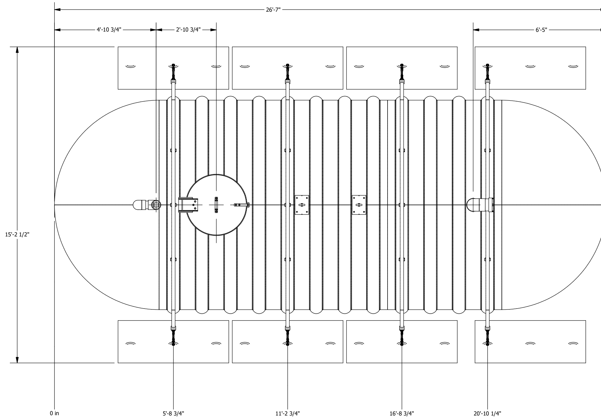
PLAN VIEW
