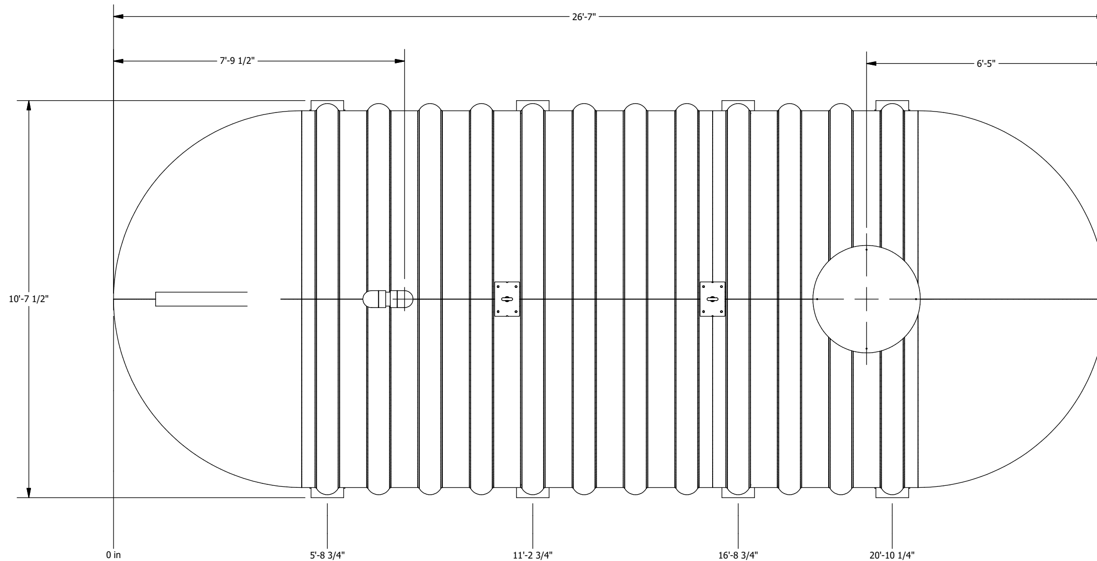
PLAN VIEW
