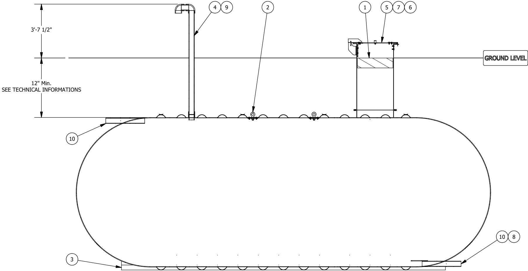
SECTION ELEVATION VIEW
