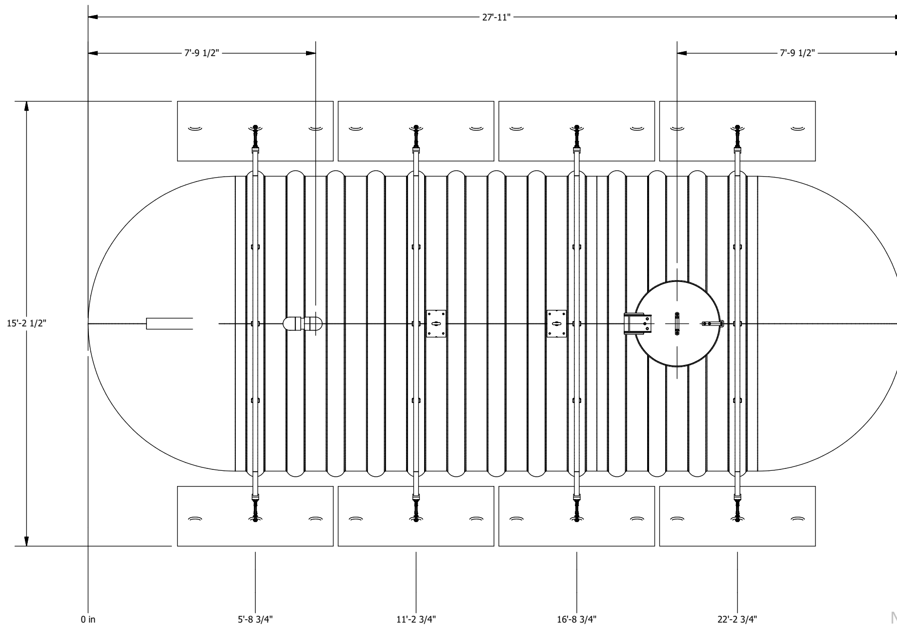
PLAN VIEW
