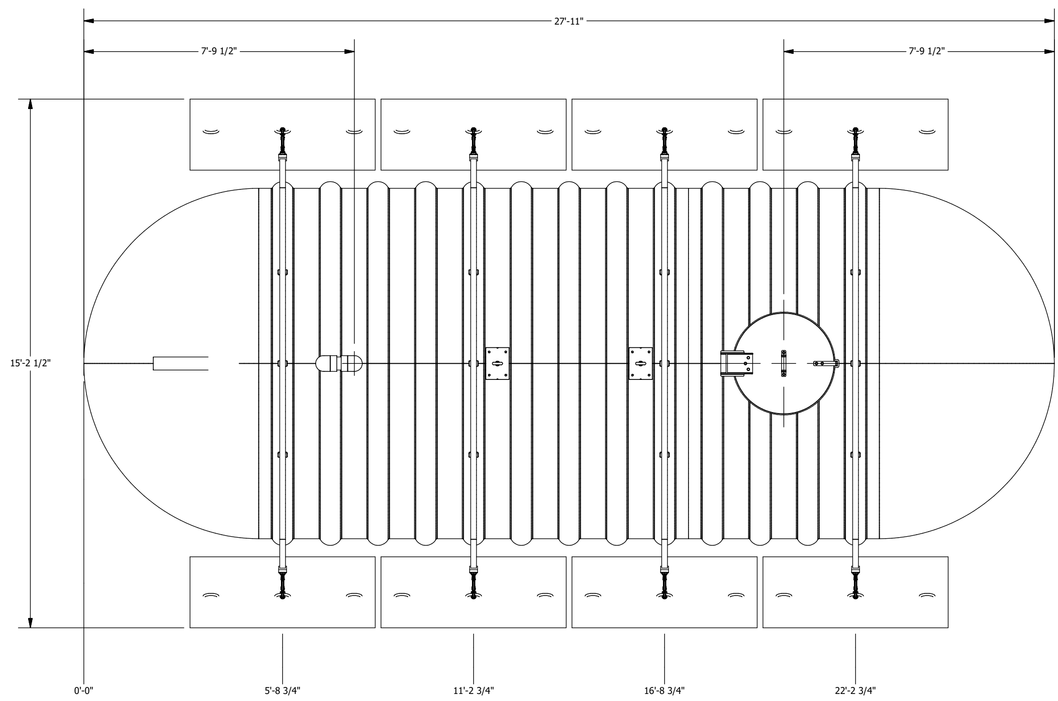
PLAN VIEW
