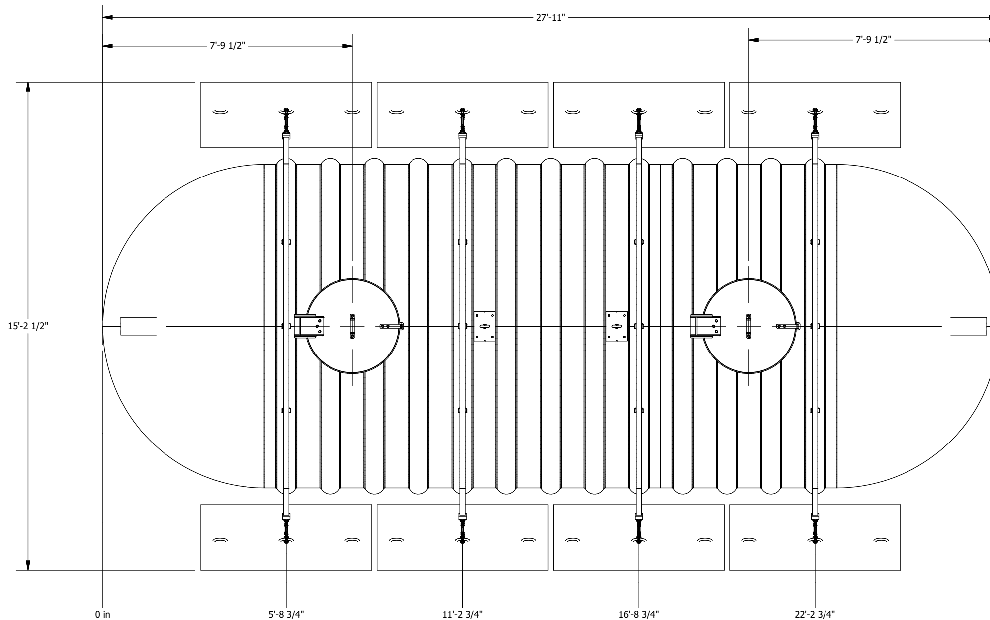
PLAN VIEW
