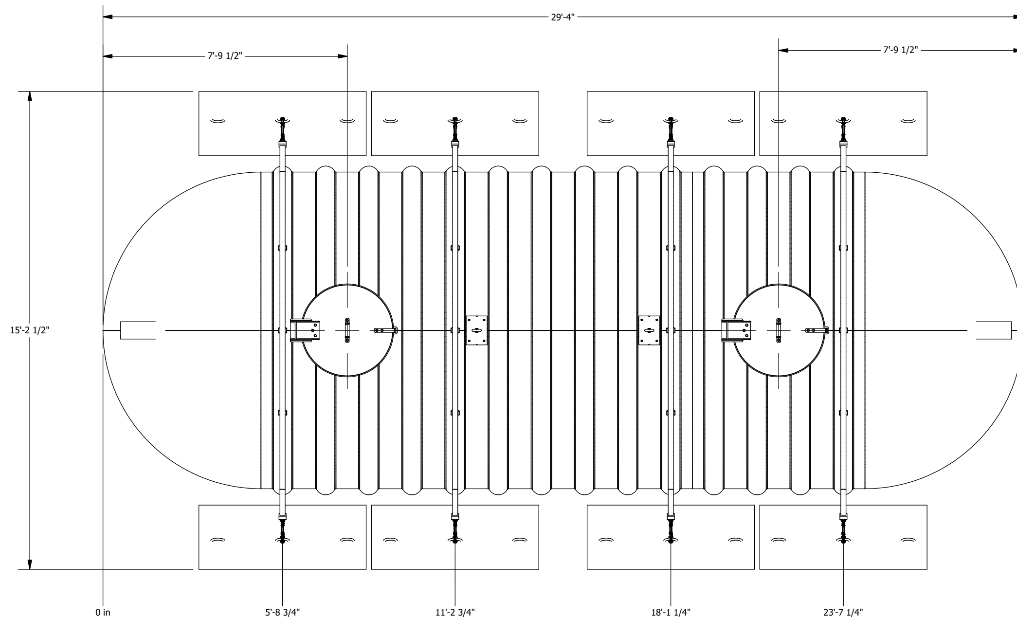
PLAN VIEW
