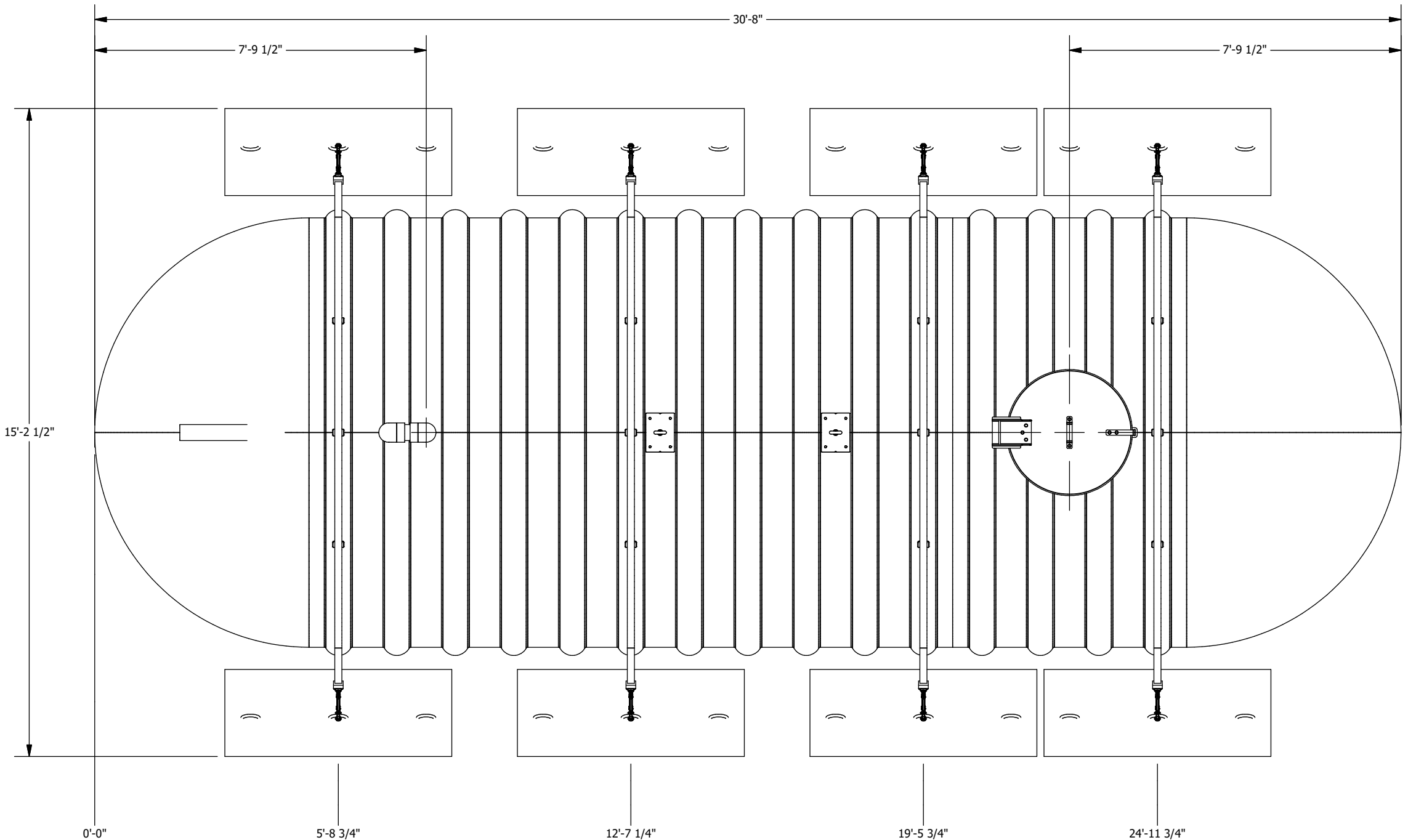
PLAN VIEW
