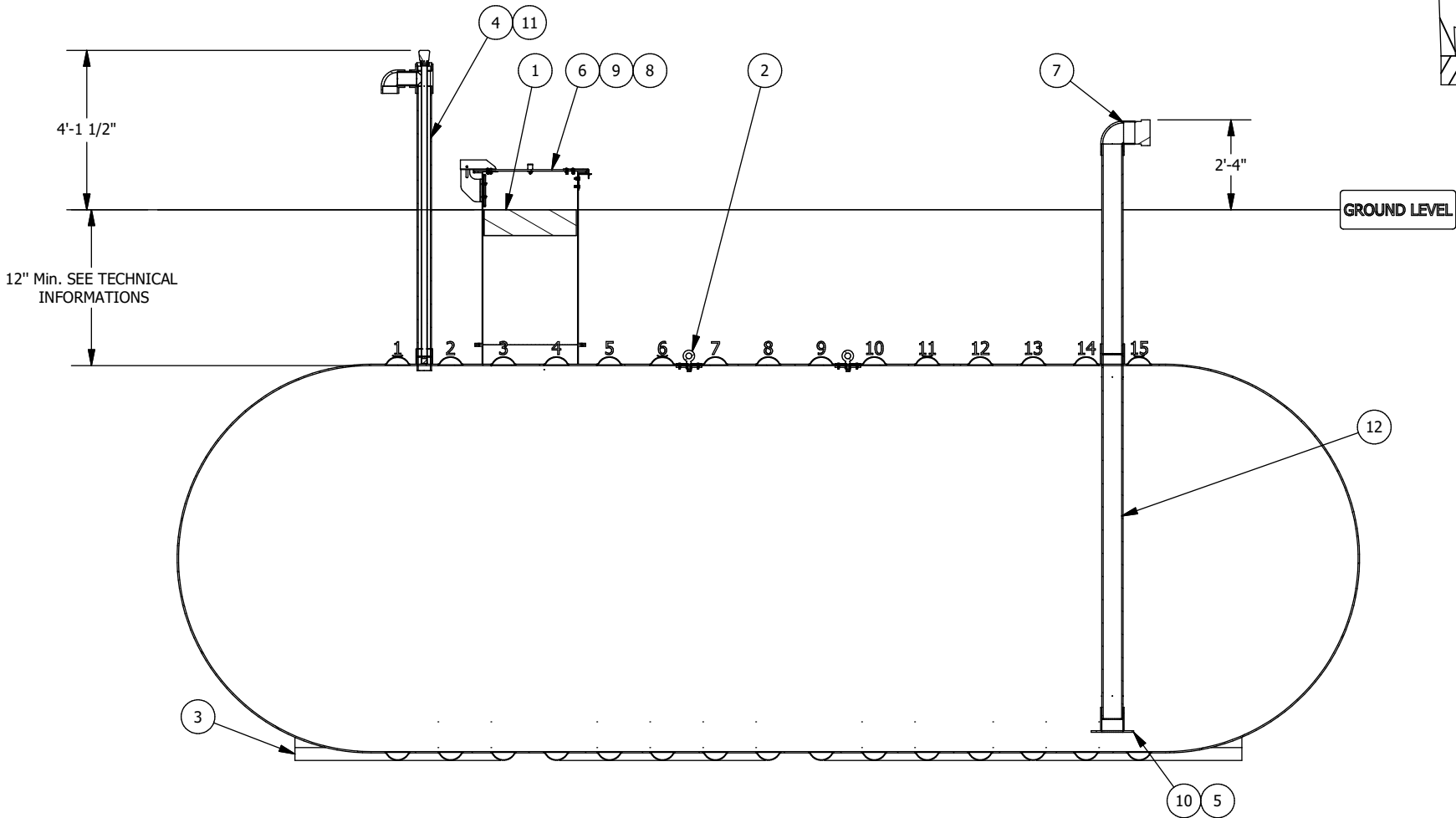
SECTION ELEVATION VIEW
