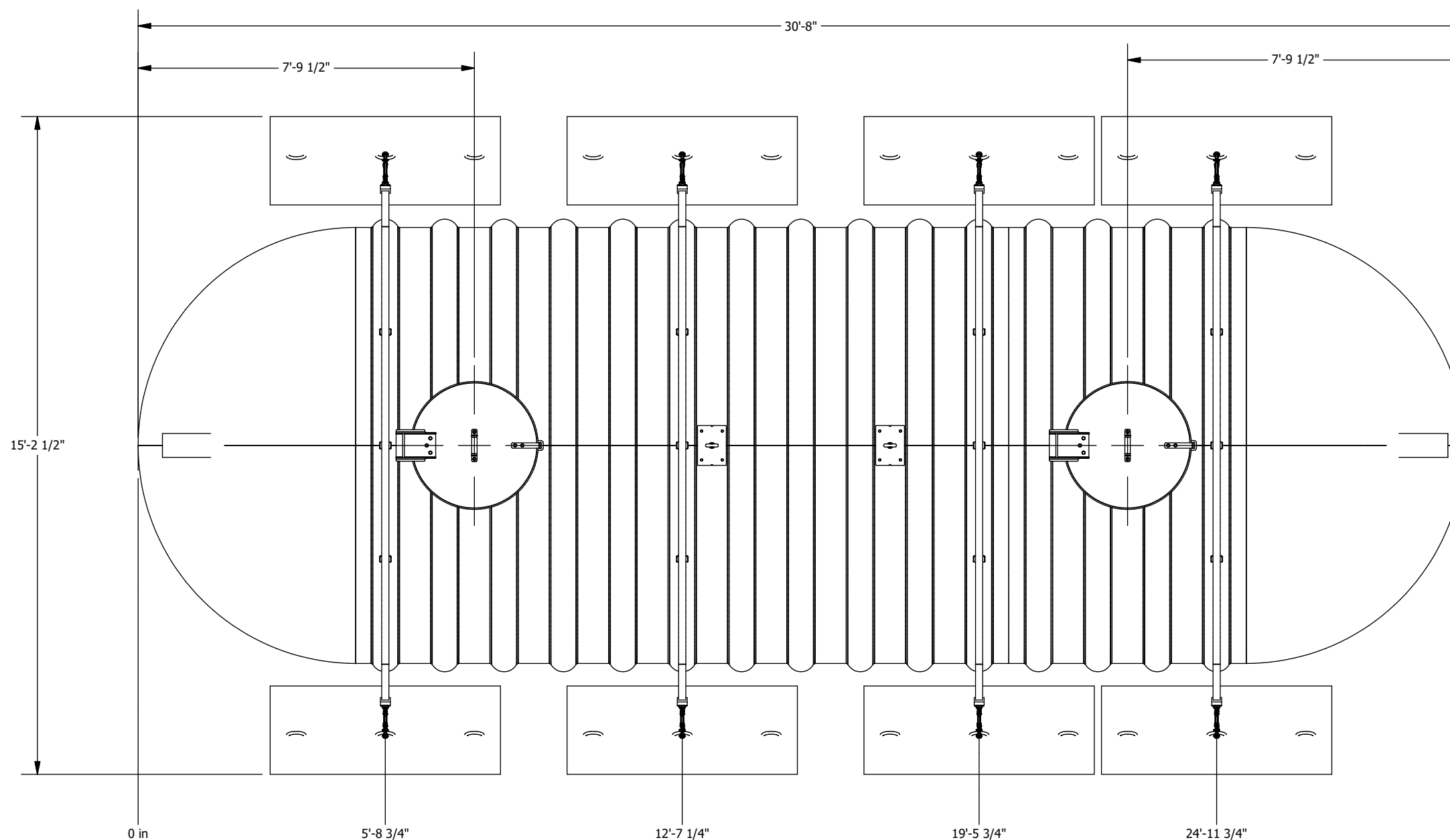
PLAN VIEW
