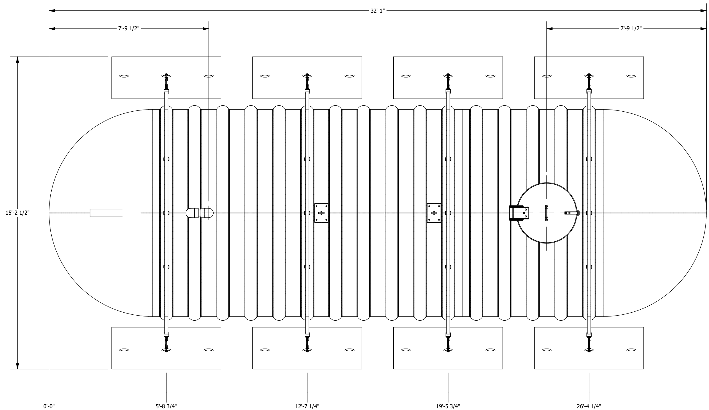
PLAN VIEW
