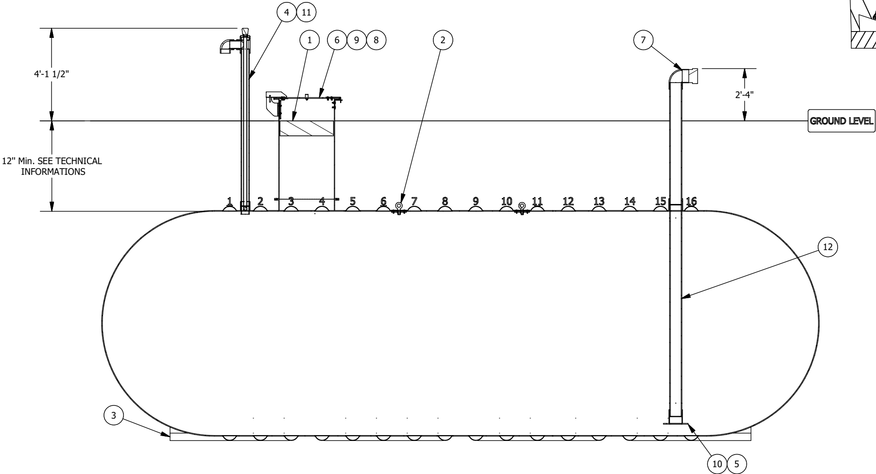
SECTION ELEVATION VIEW
