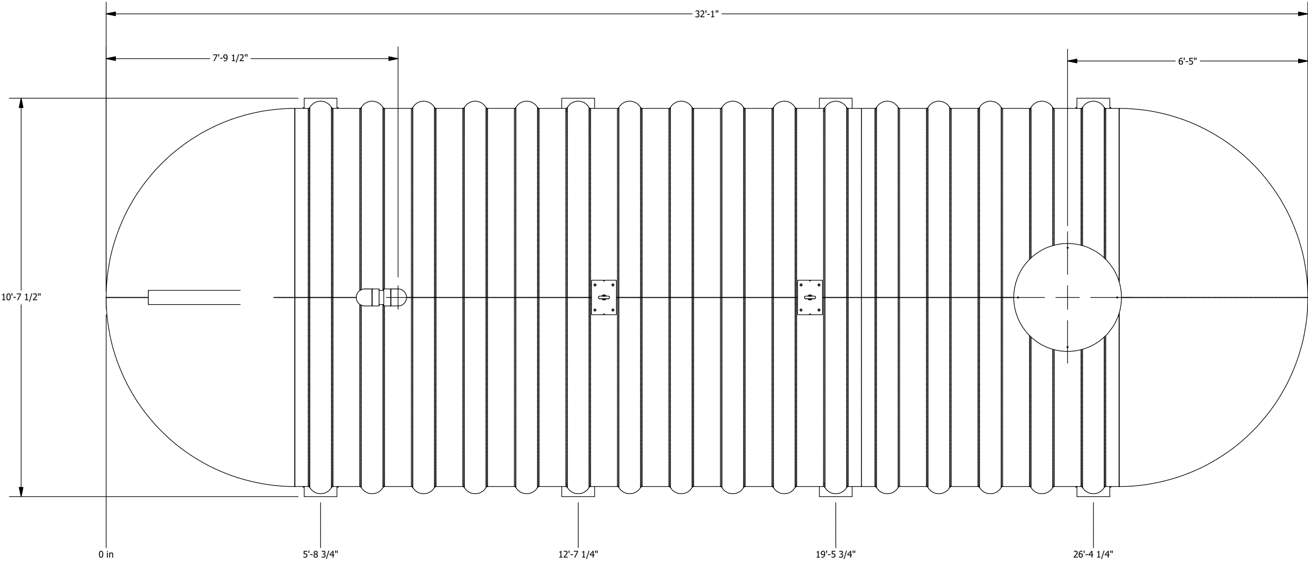
PLAN VIEW
