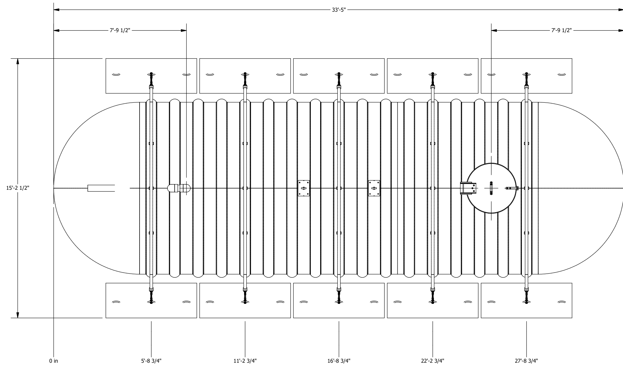
PLAN VIEW
