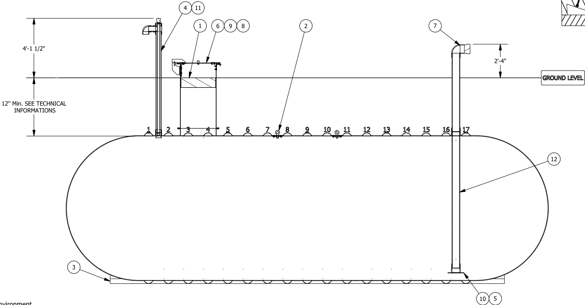
SECTION ELEVATION VIEW
