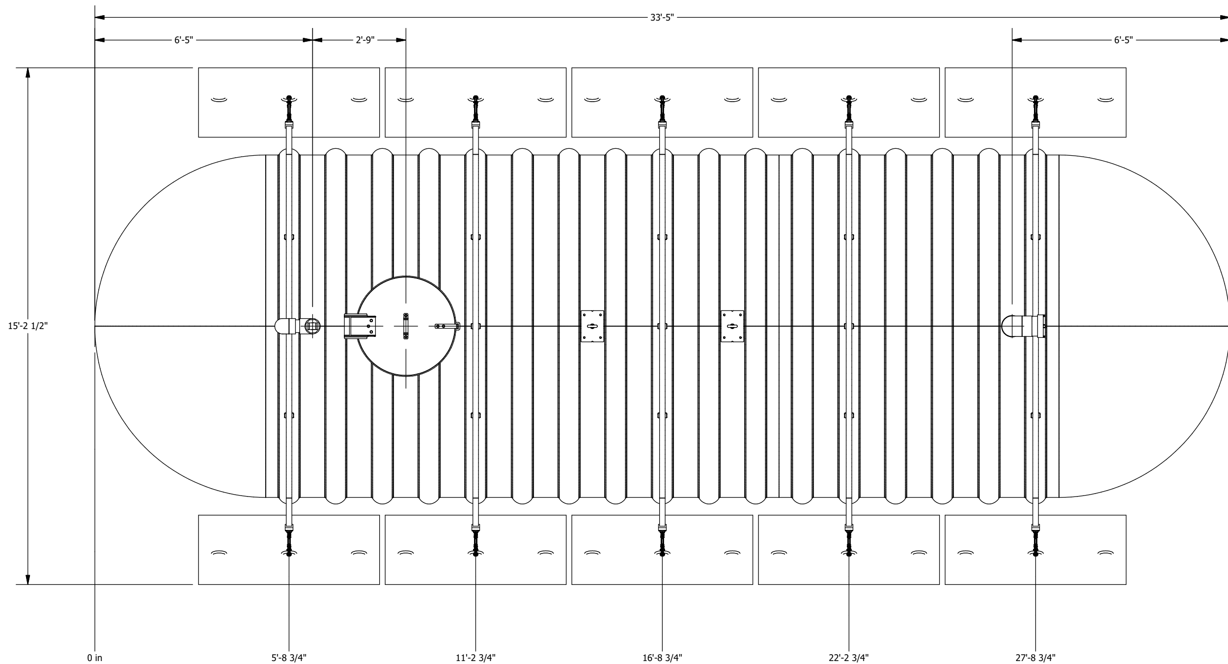
PLAN VIEW
