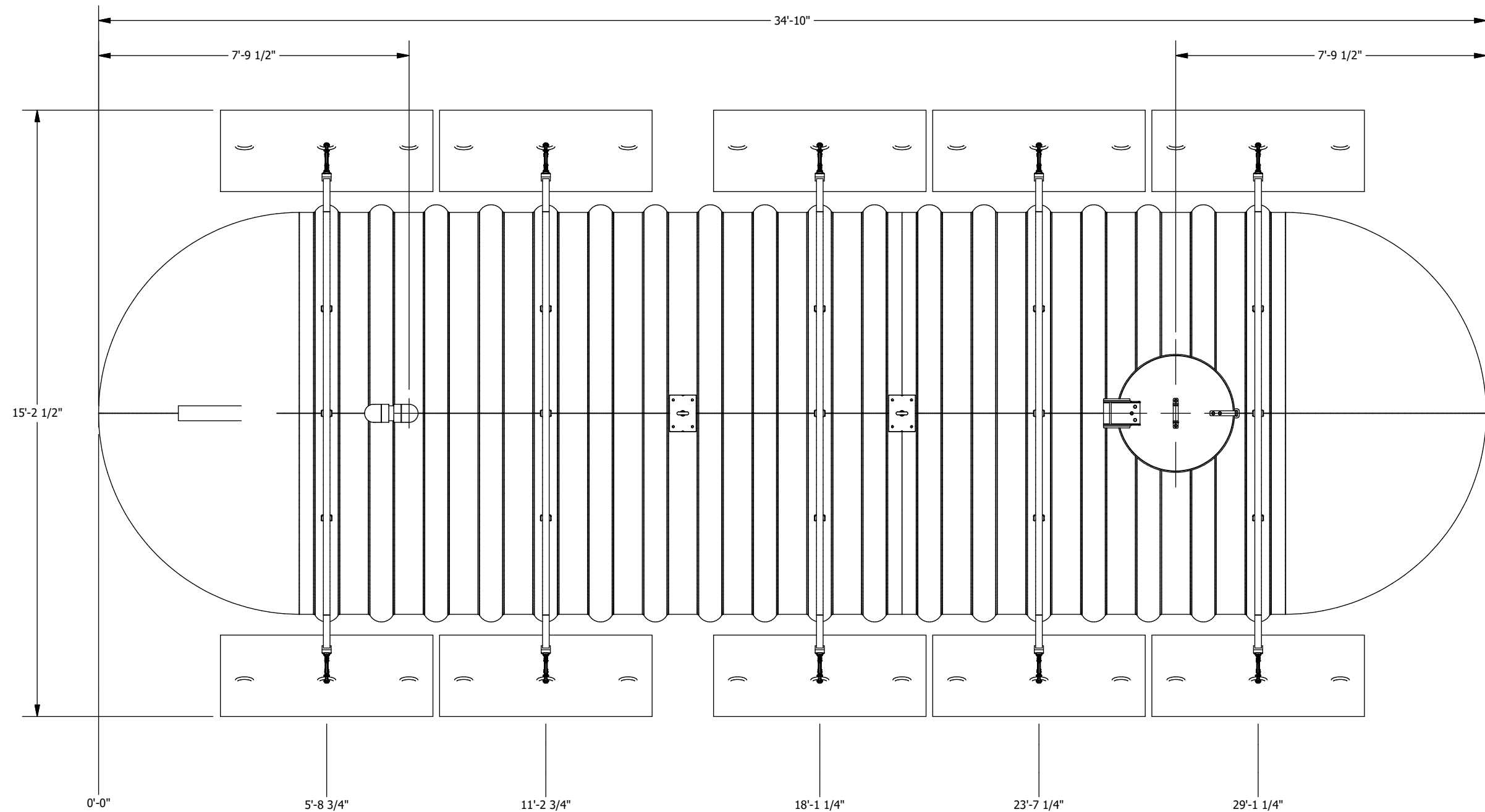
PLAN VIEW
