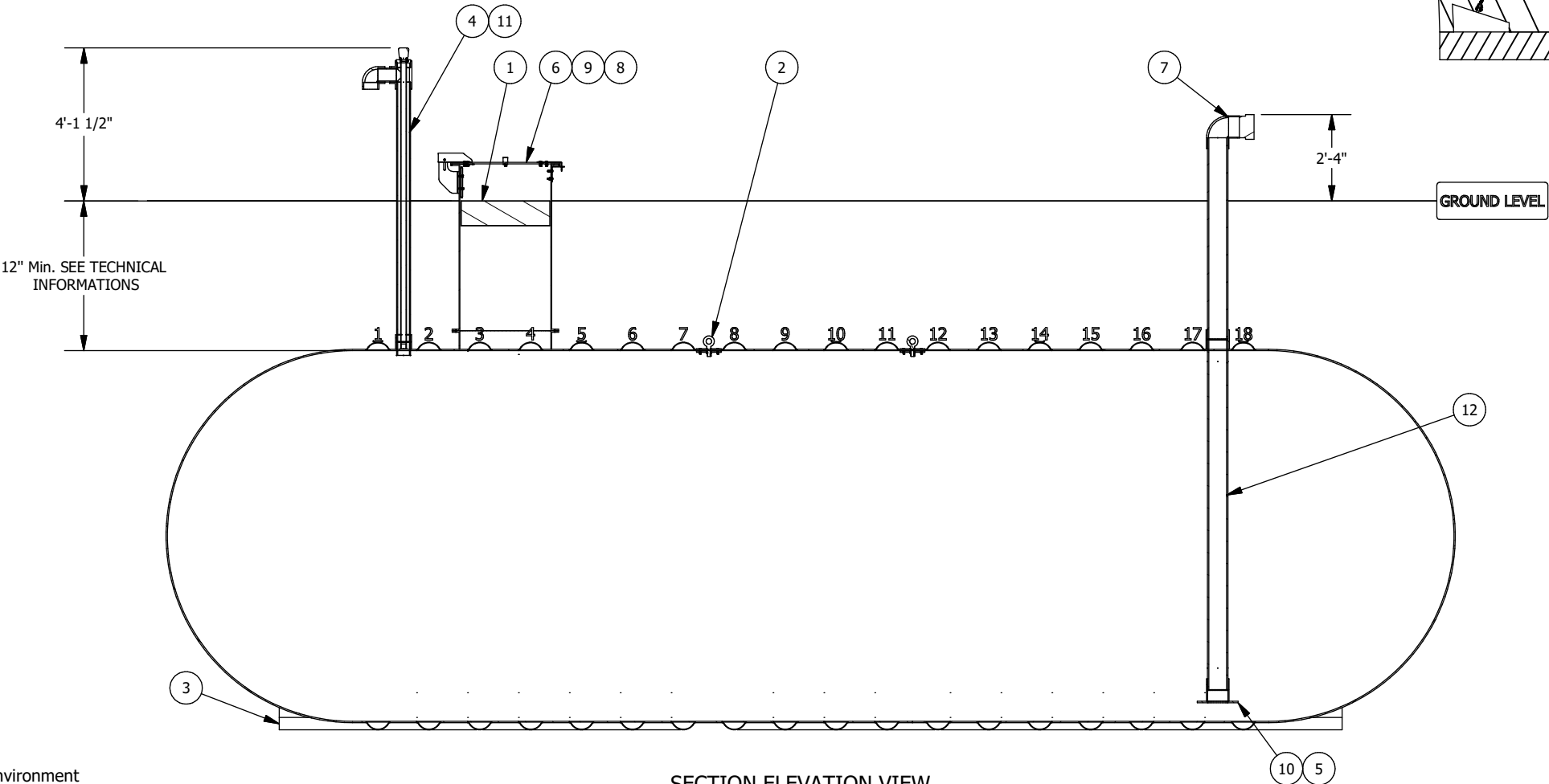
SECTION ELEVATION VIEW
