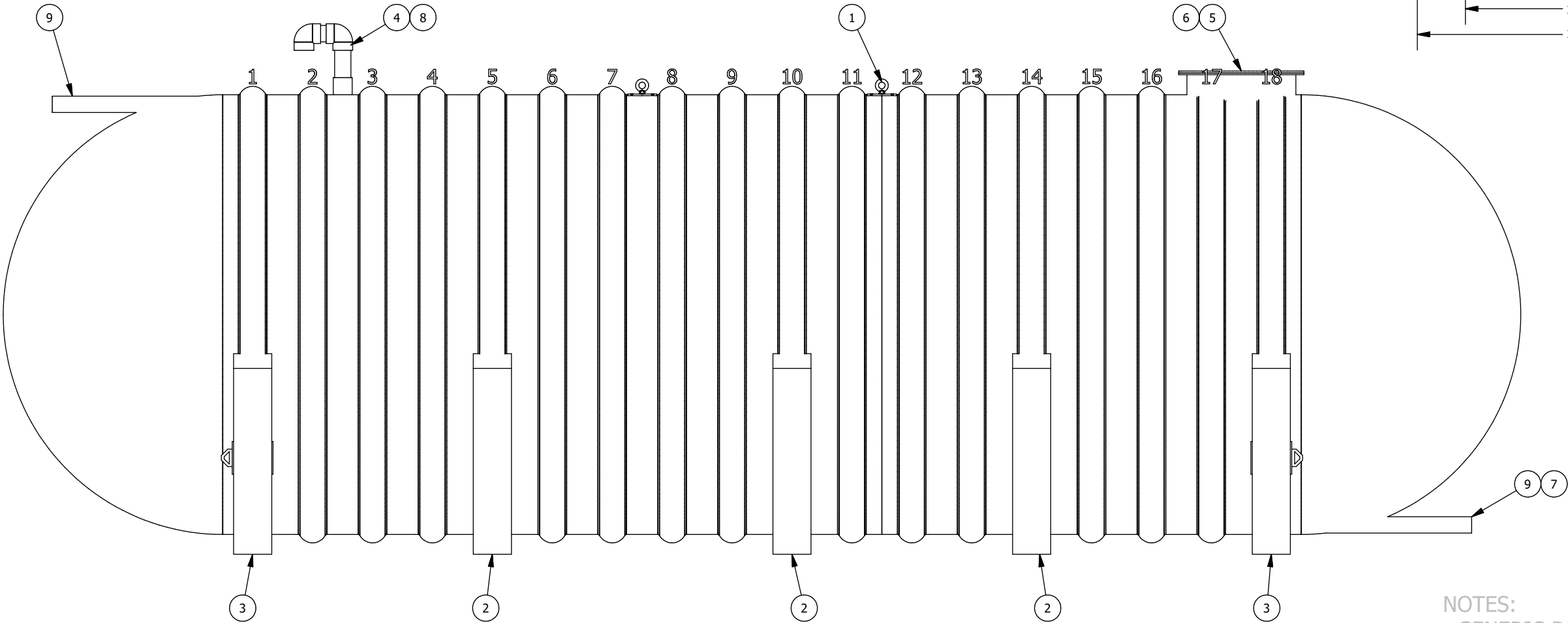
ELEVATION VIEW
