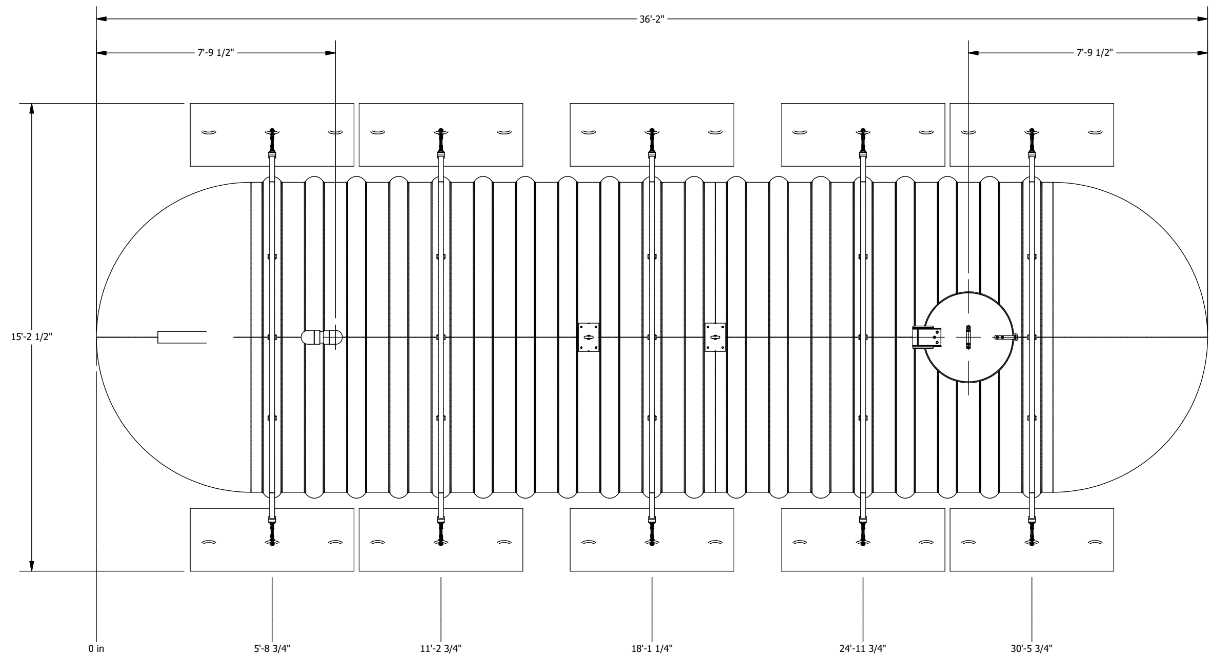
PLAN VIEW
