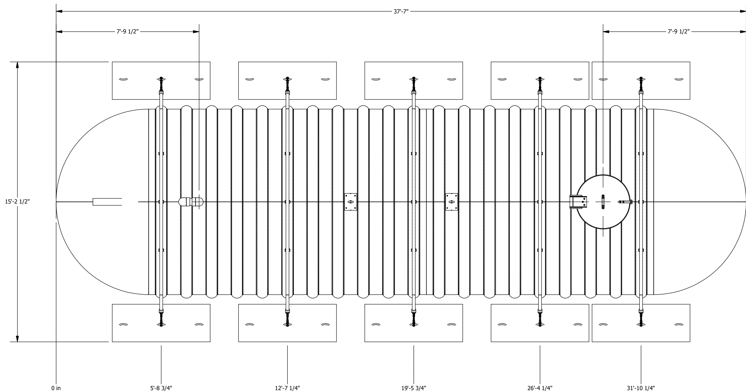
PLAN VIEW
